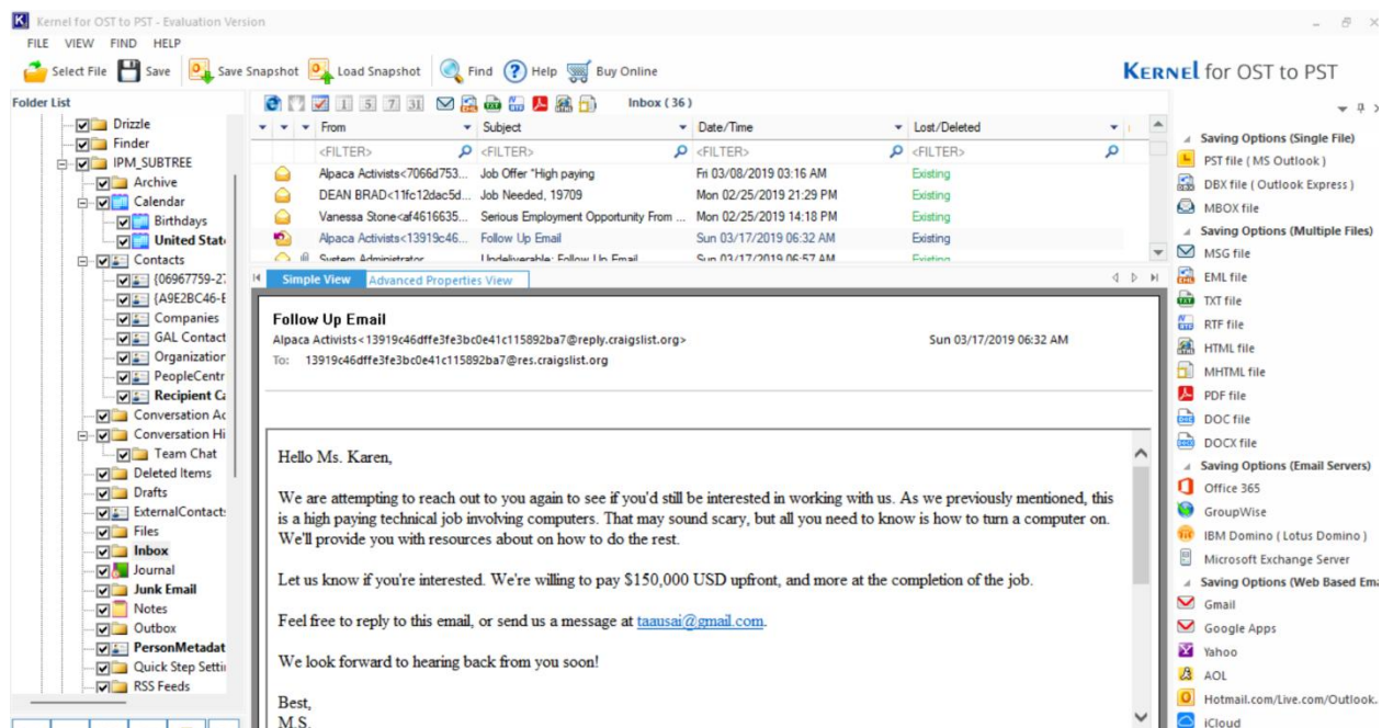
Fig2.6_initial
