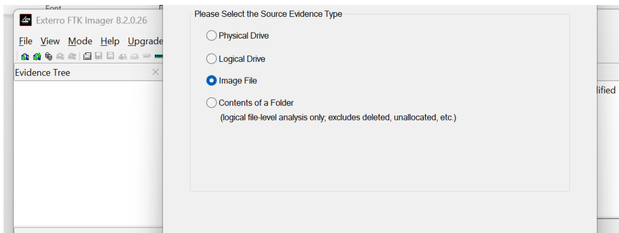
Fig1_ftk_imager
