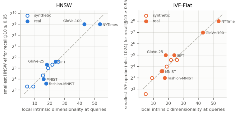
Figure 2. Smallest setting reaching recall@10 of 0.95 against LID for all twelve datasets. Filled points are real, hollow points synthetic; the dashed line is the fitted model.
