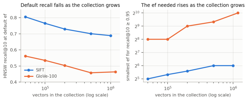
Figure 3. SIFT and GloVe-100 at five collection sizes. Left: HNSW recall at the default ef. Right: the smallest ef reaching recall 0.95 (log scale).
