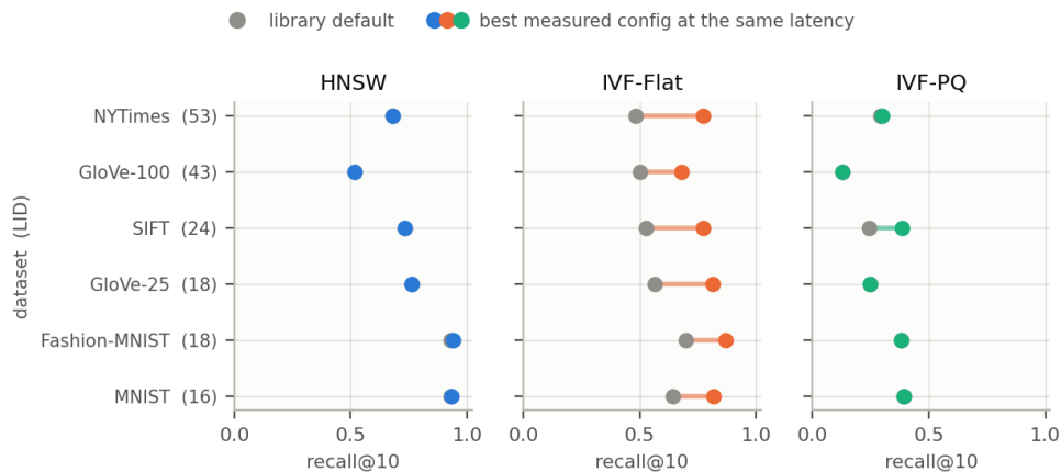
Figure 1. Default recall (gray) against the best measured configuration at the same latency (colored), k = 10 . Rows are sorted by LID, shown in parentheses.
