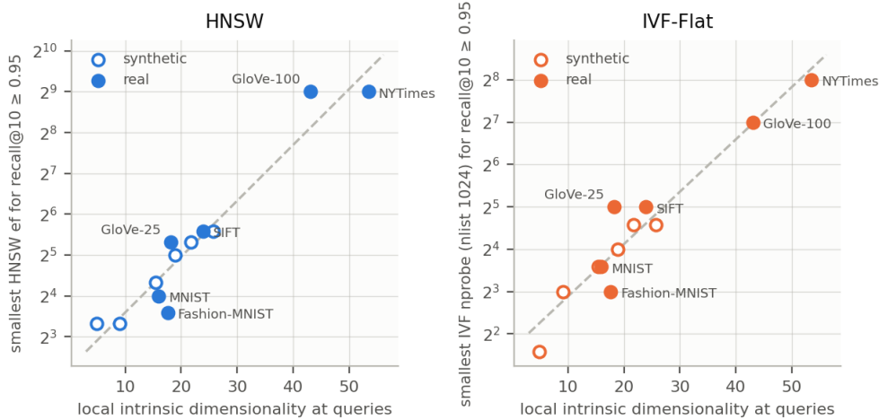
Figure 1. Smallest setting reaching recall@10 of 0.95 against LID, twelve datasets. Filled points are real, hollow points synthetic; the dashed line is the fitted model (log scale).
