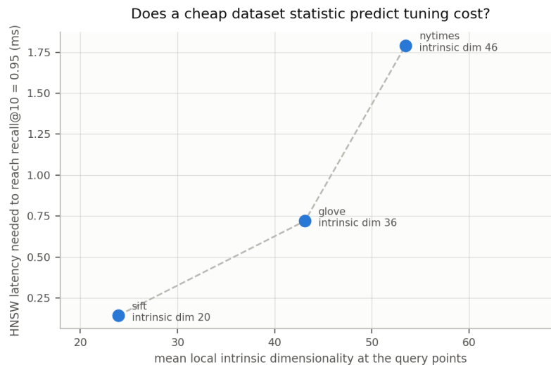
Figure 3. Query-point local intrinsic dimensionality against the HNSW latency needed to reach recall 0.95. Three points, monotone, not yet a fitted model.
