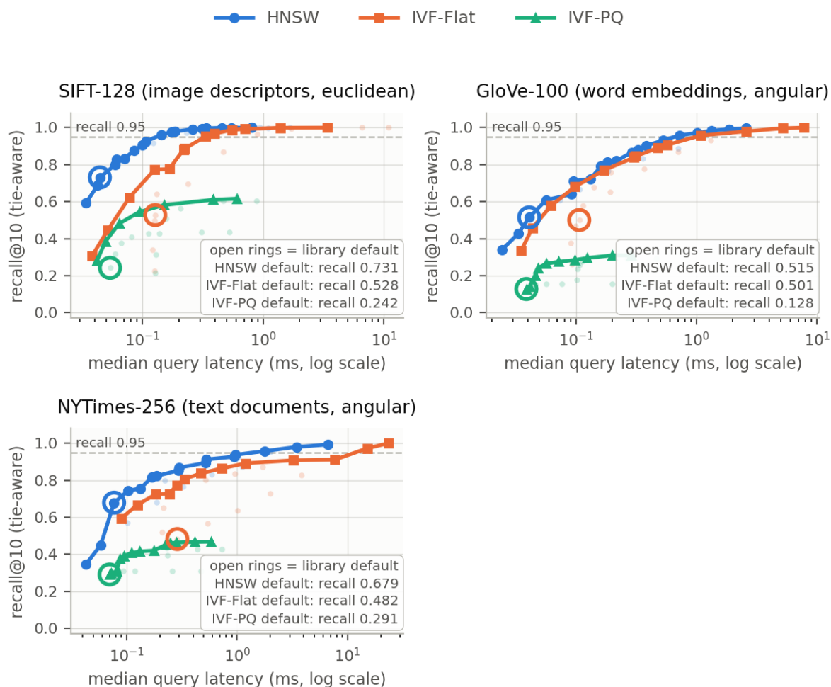
Figure 1. Measured recall-latency frontiers for all three index families on all three datasets. Faint dots are individual measured configurations; solid lines are the Pareto frontier; open rings mark each library's default configuration.
