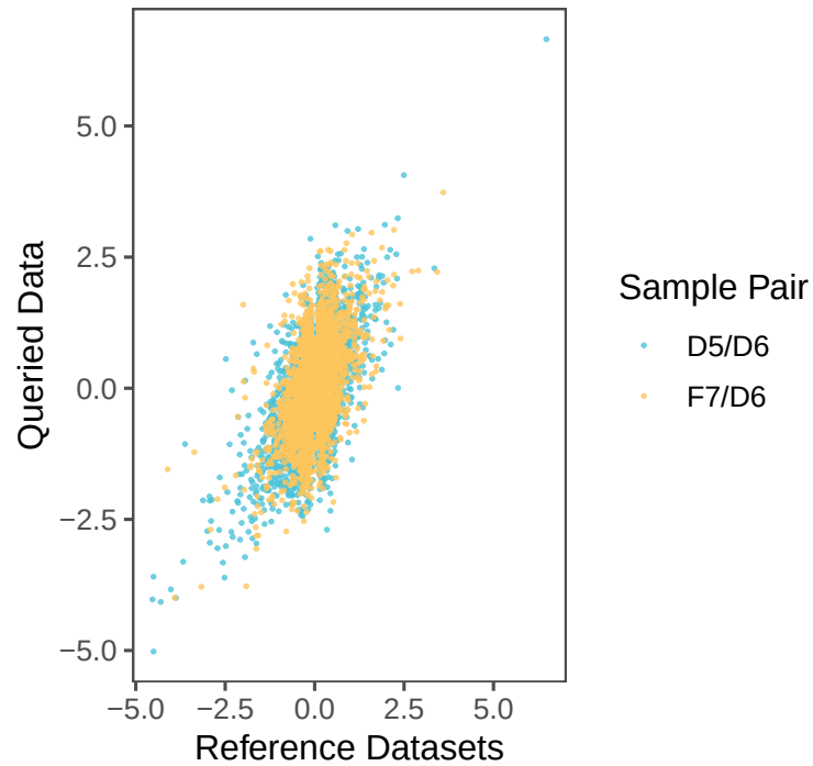
Correlation: 0.590 (N = 12259)
