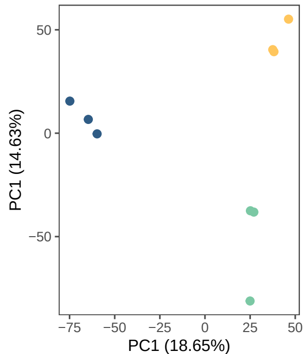
SNR: 13.739 (N = 13639)
