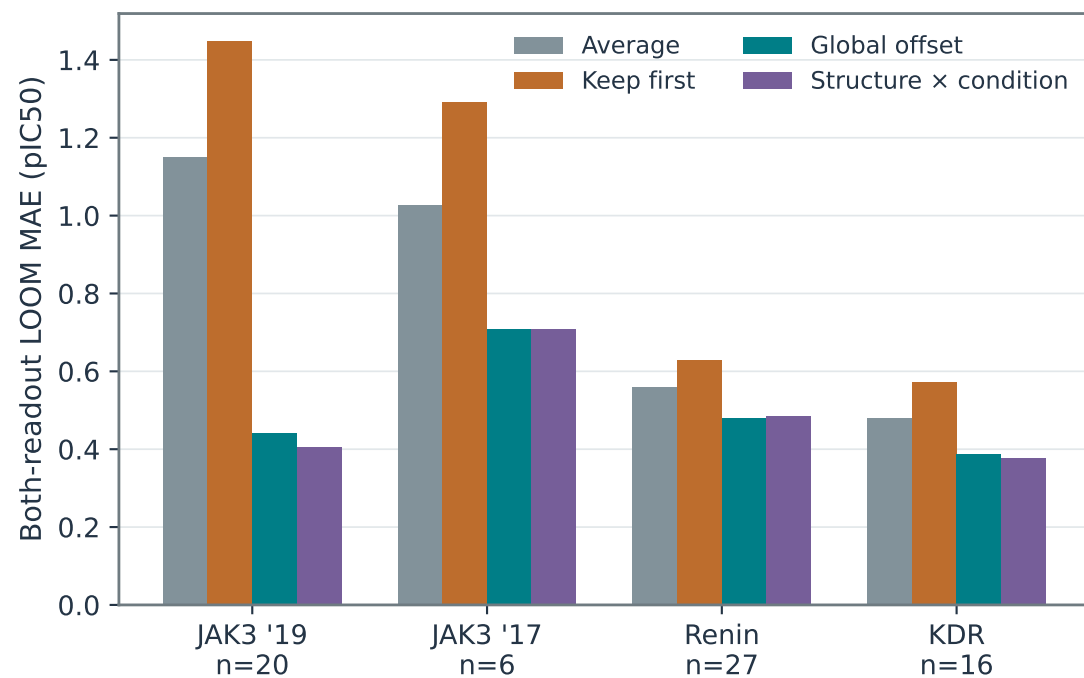
c Same-molecule record-policy baselines
