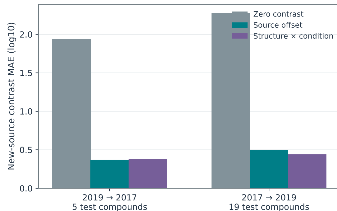
d JAK3 paper transfer tests calibration
