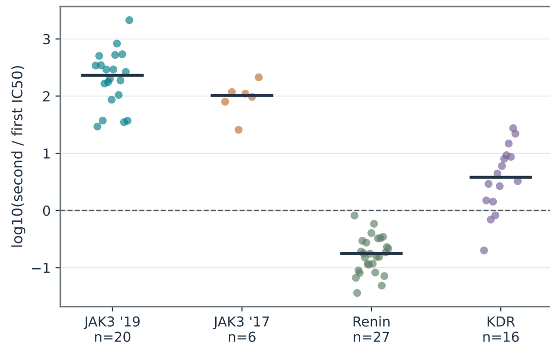
a Measured contrasts include source-level shifts
