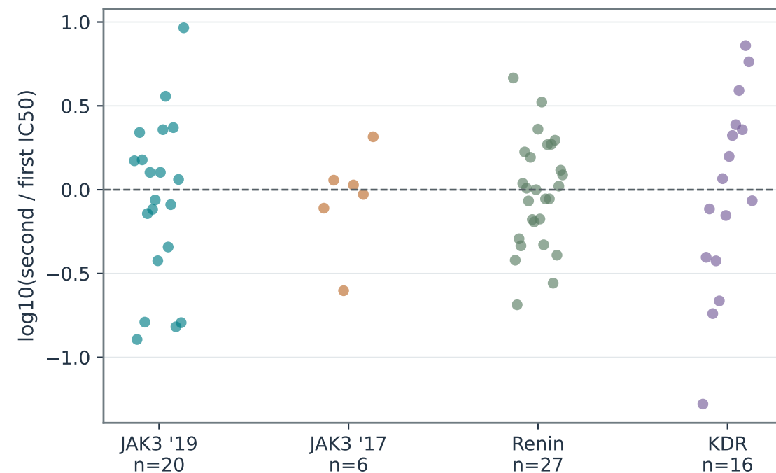
b Median-centred residuals retain molecular variation
