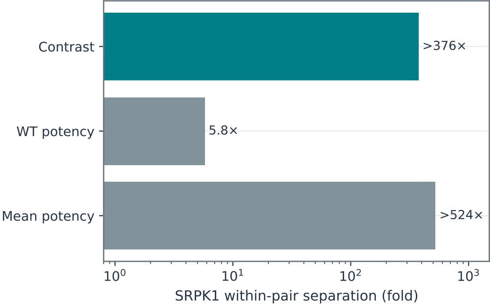
c Cross-target endpoint in the same patent
