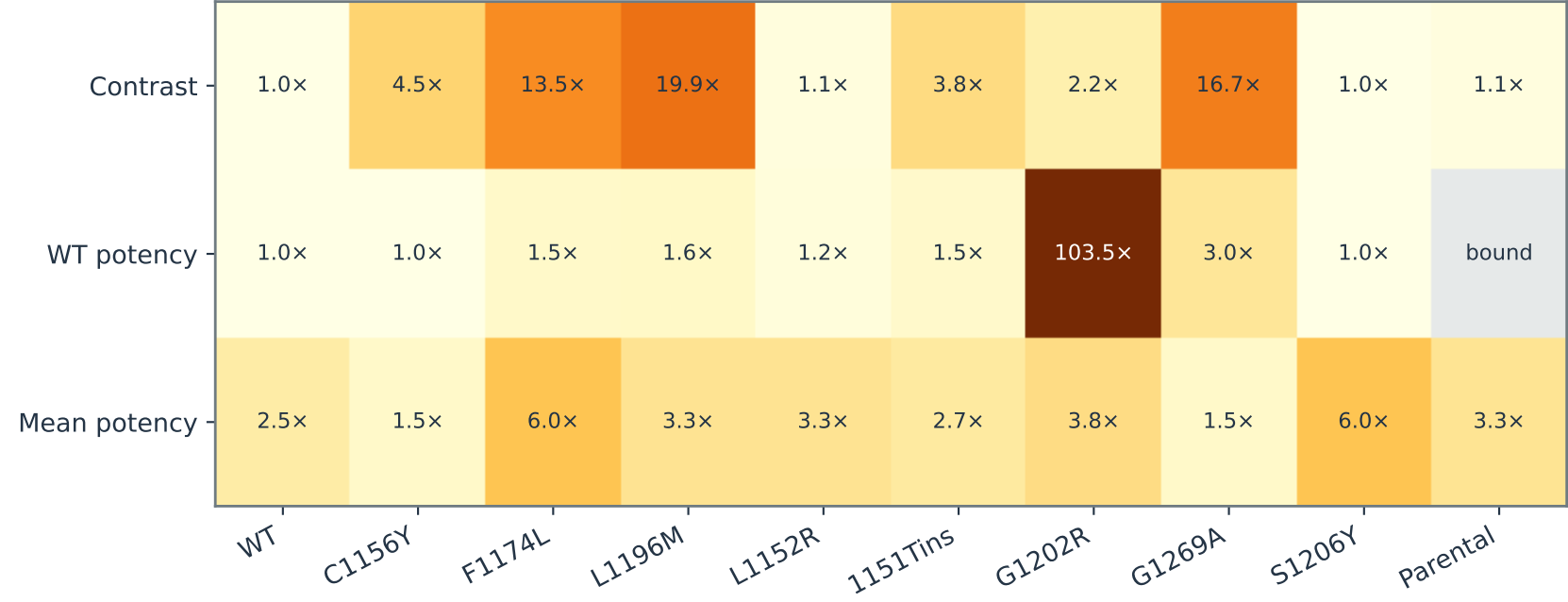
b Equal two-compound budget: within-pair separation
