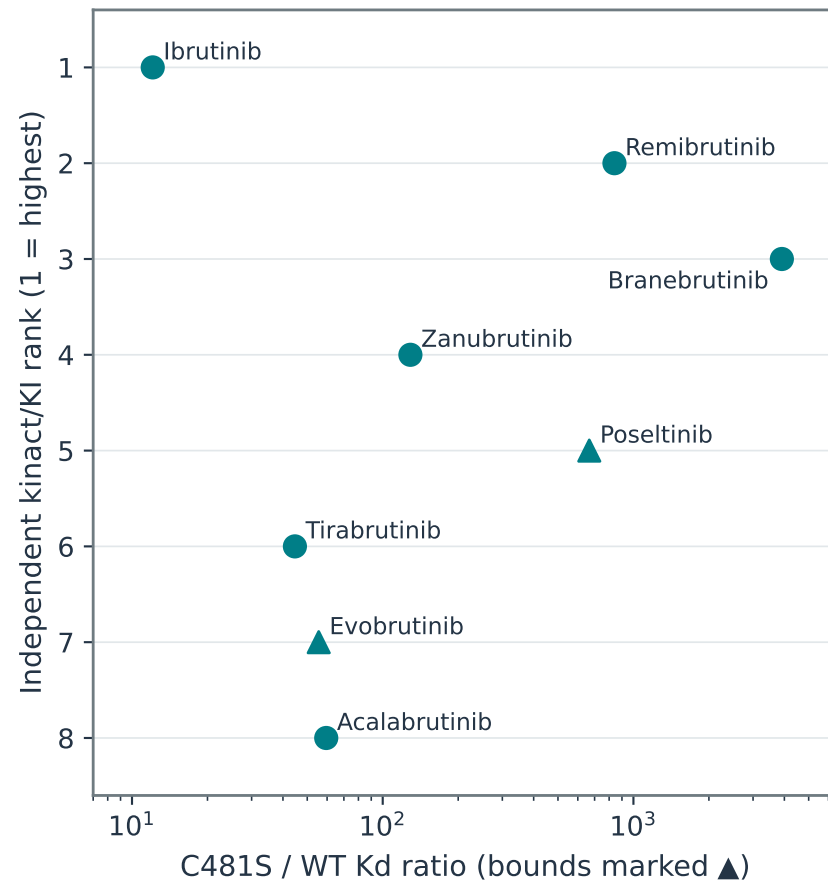
b Affinity shift is not a kinetic rank
