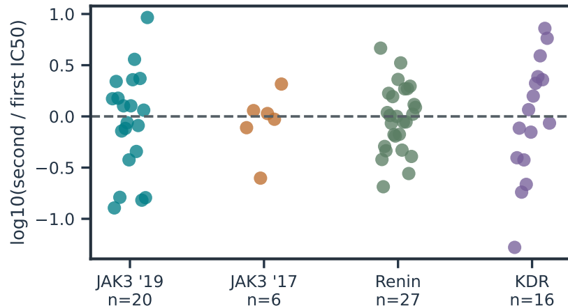
B Residual molecular variation
