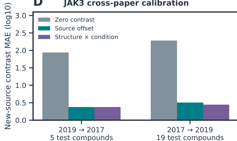
D JAK3 cross-paper calibration
