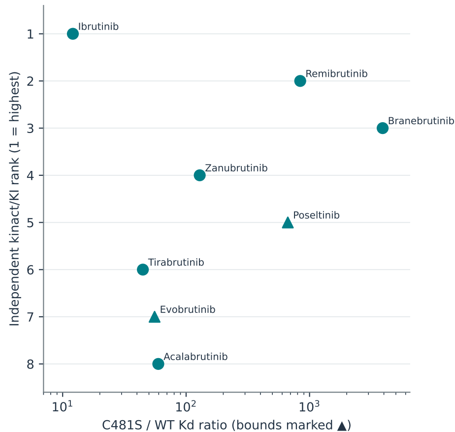
b Affinity shift is not a kinetic rank
