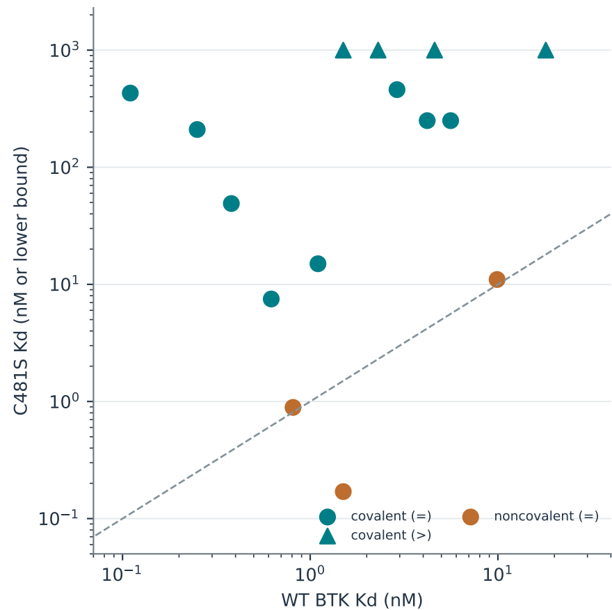
a Corrected BTK mutation contrasts
