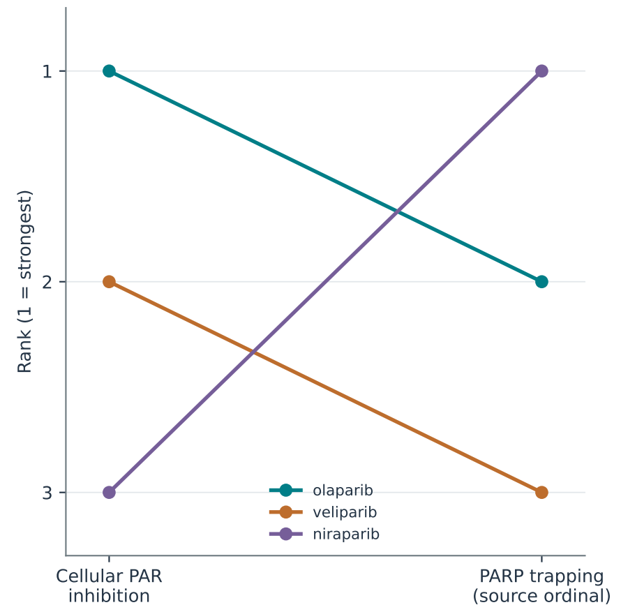
c Published PARP source-ordinal rank inversion
