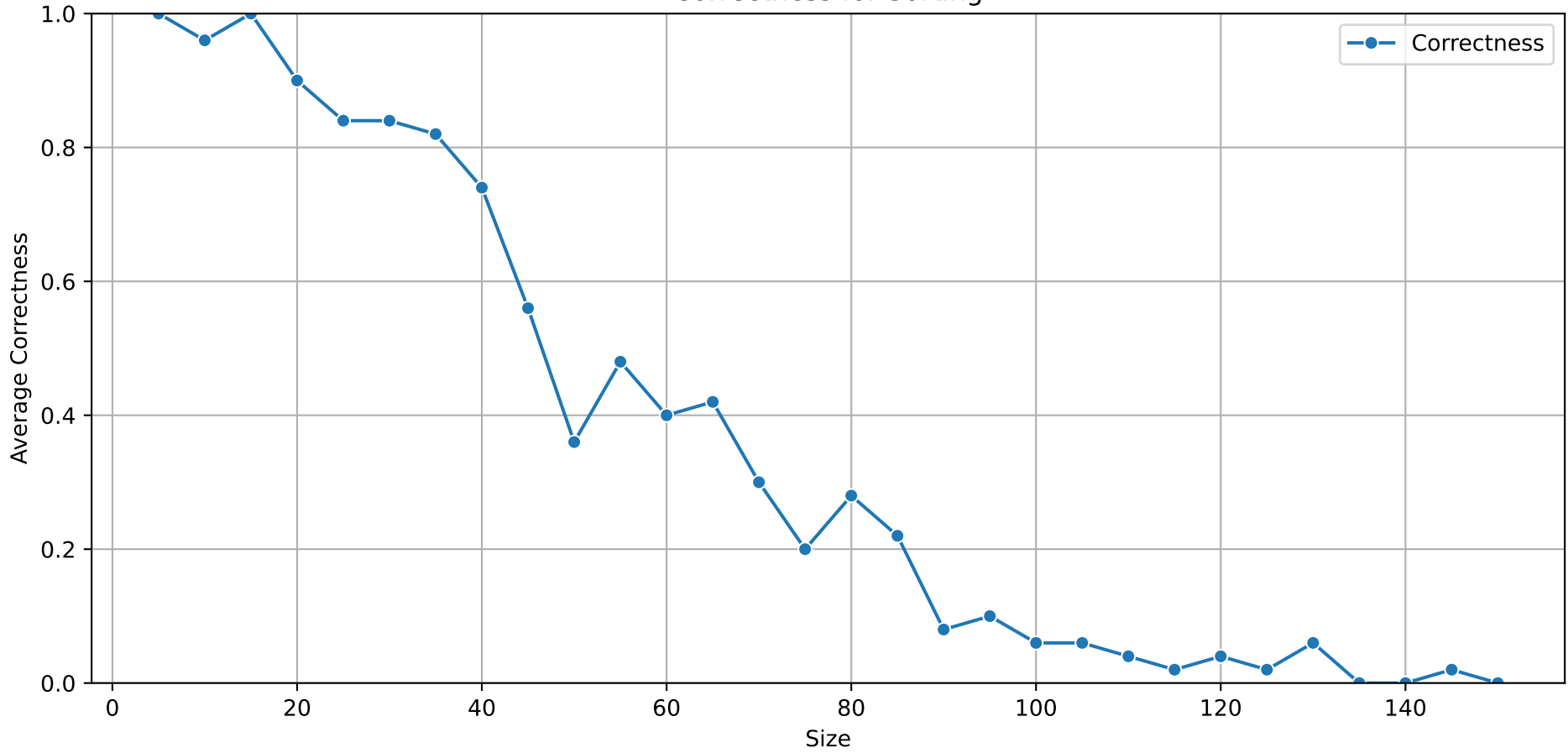
Inverse Multiplication for Sorting
