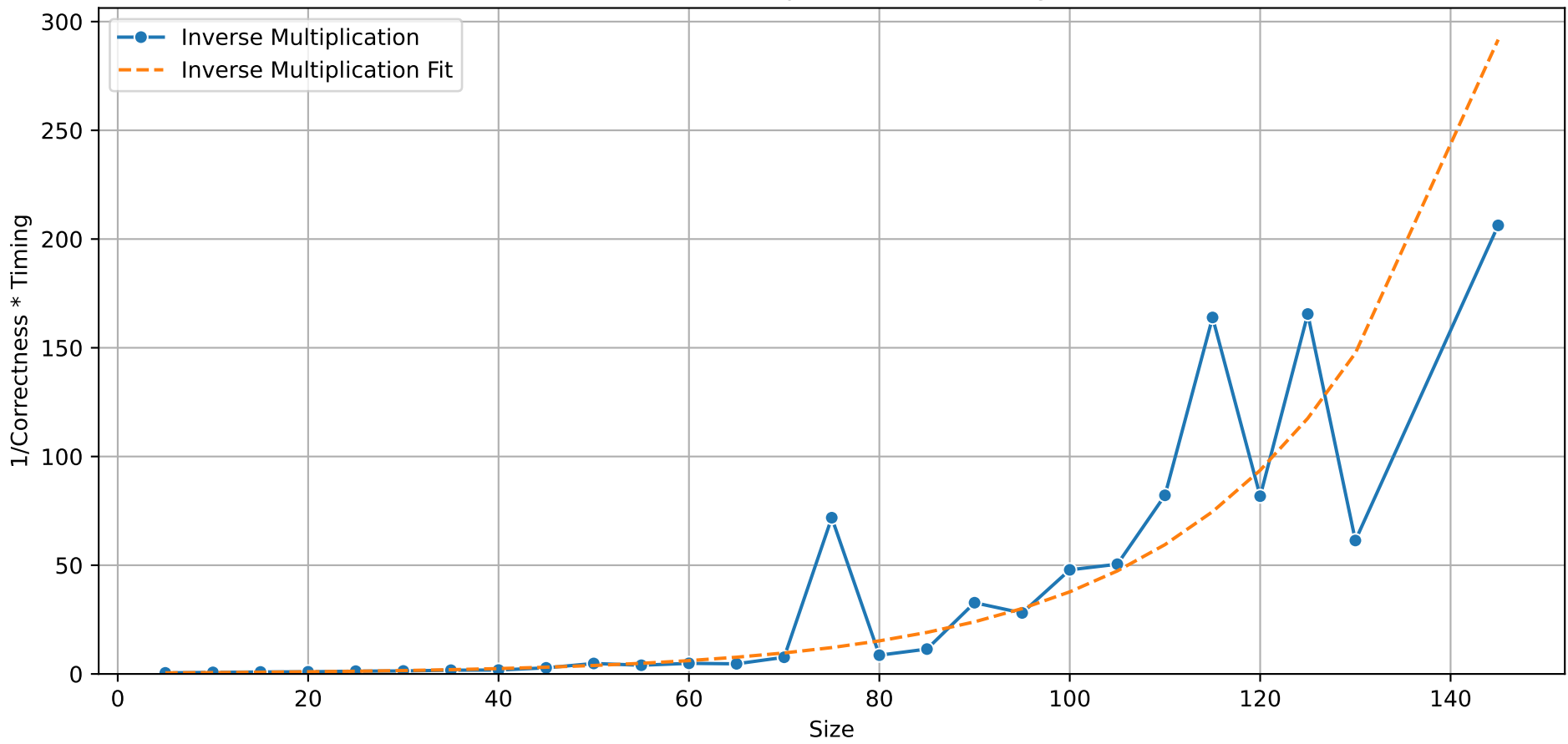
Inverse Multiplication for Sorting
