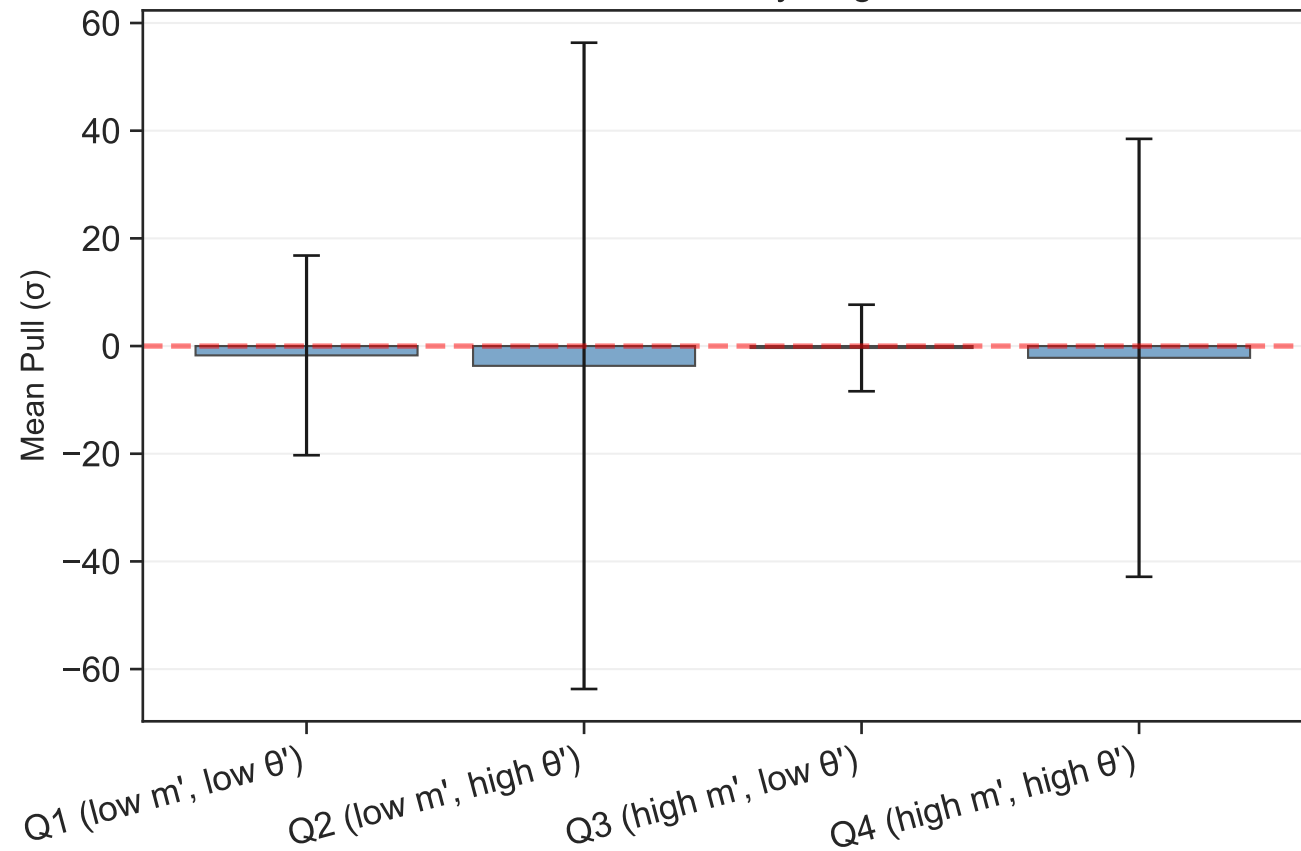
Pull Statistics by Region
