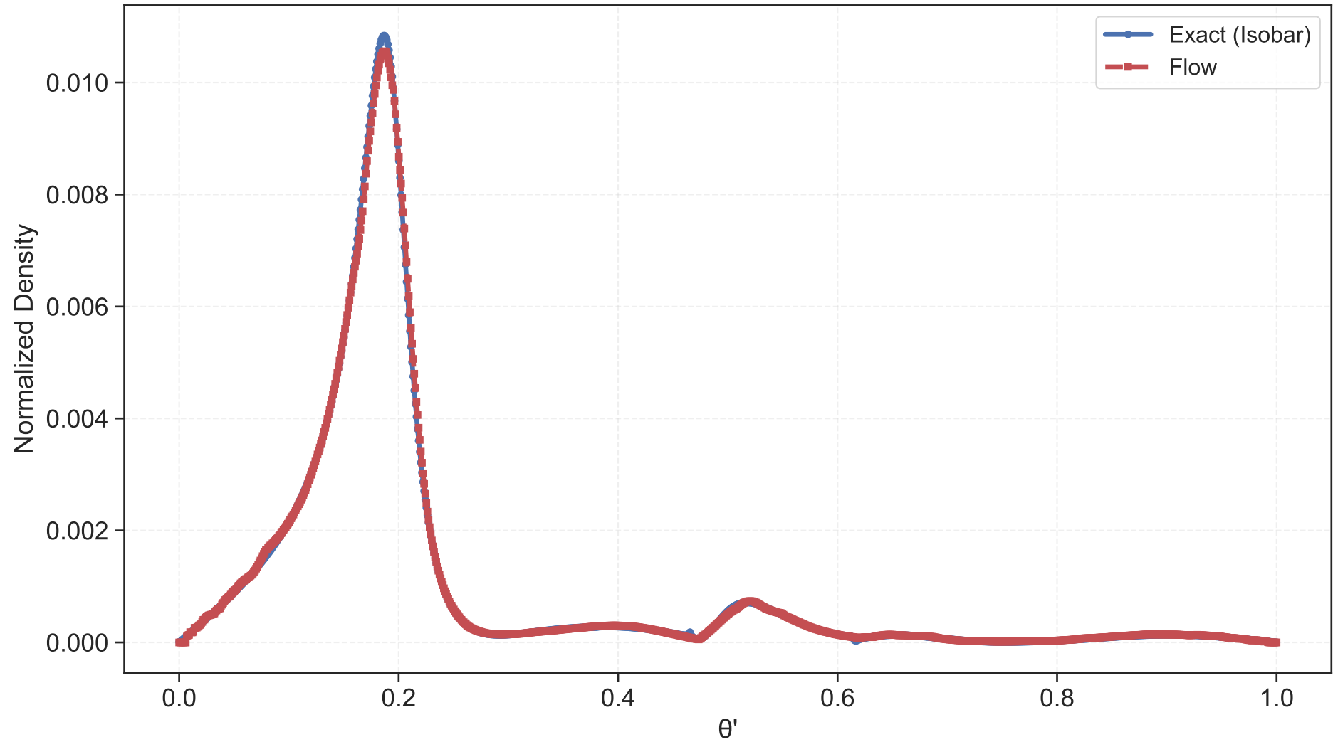
Density vs \theta' at m' = 0.5000
