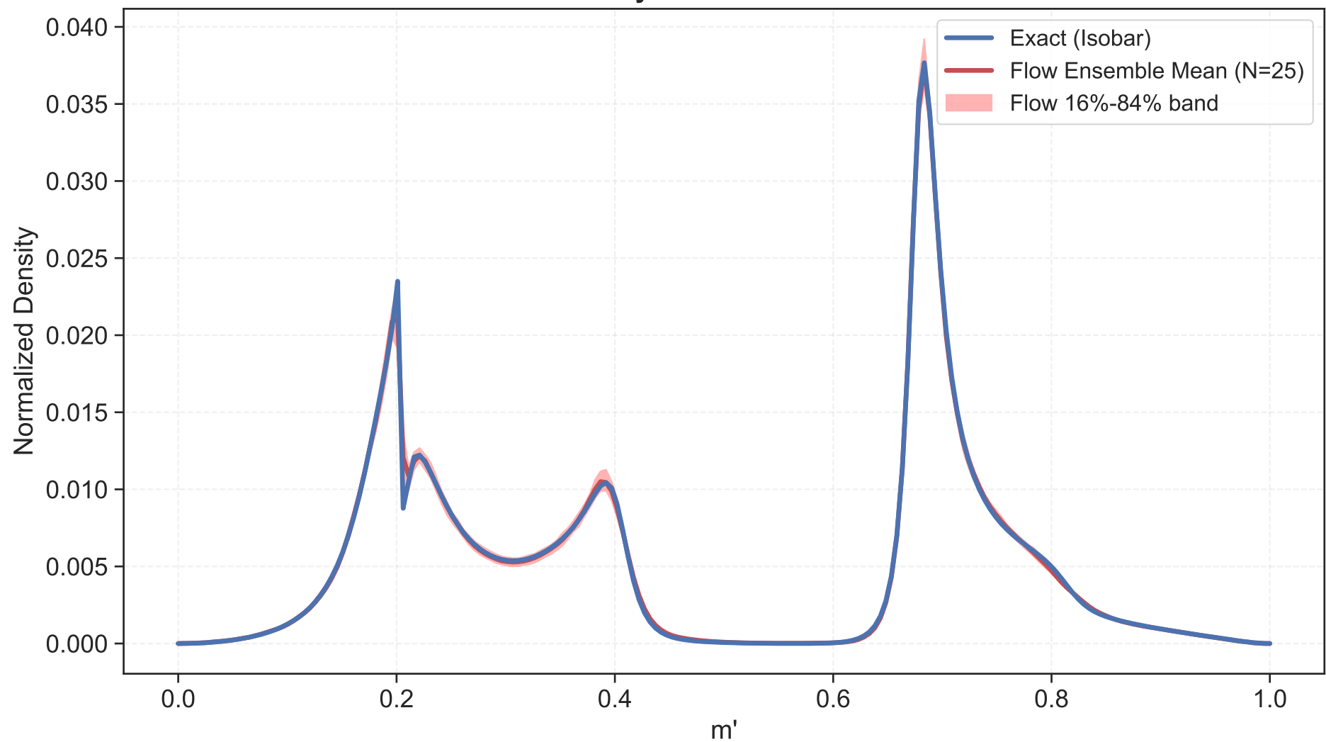
Density vs m' at \theta' = 0.3000
