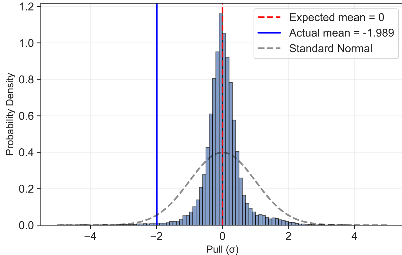
Combined Ensemble Pull Distribution
