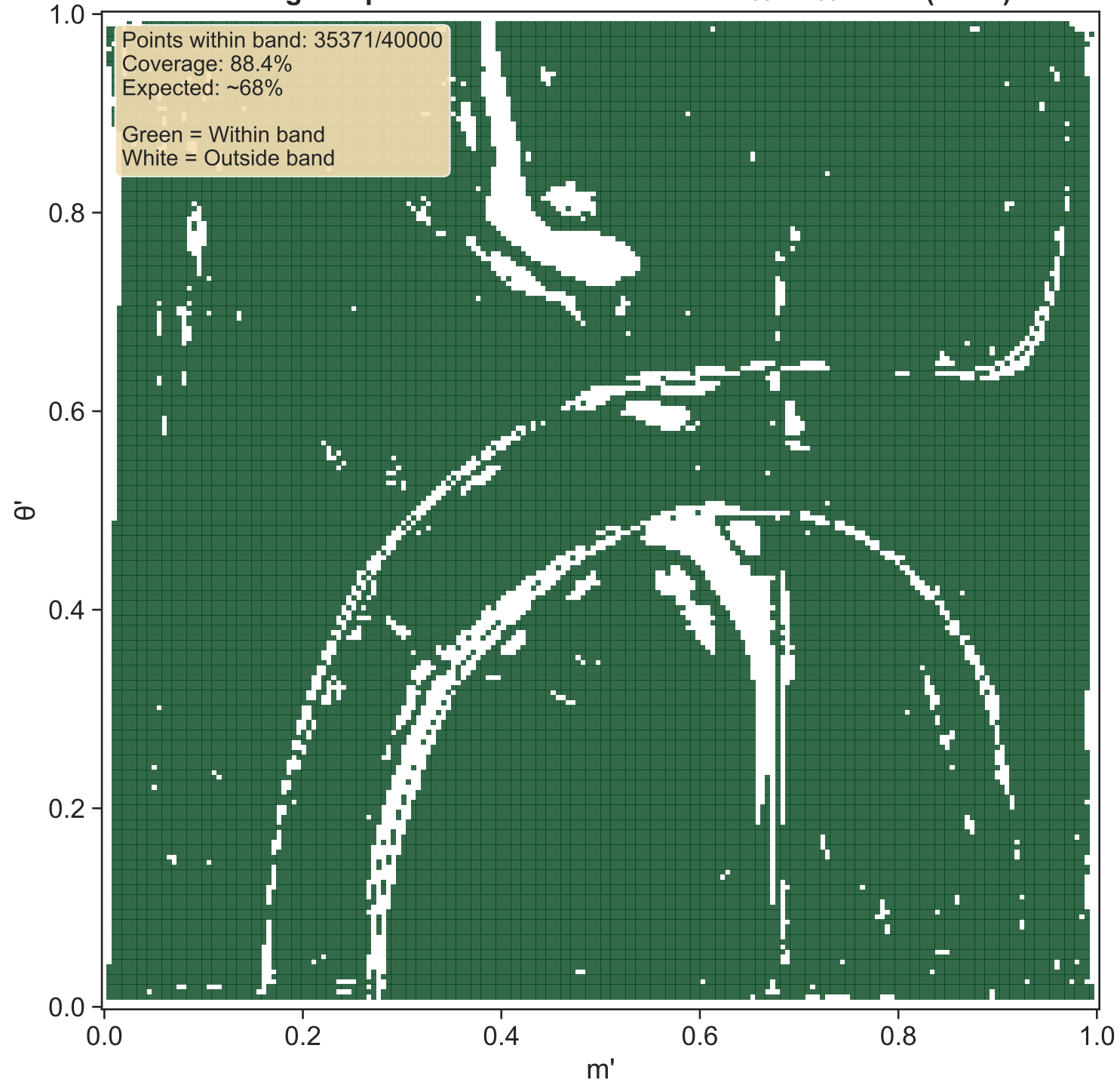
Coverage Map: Exact Within Ensemble 16%-84% Band (N=25)
