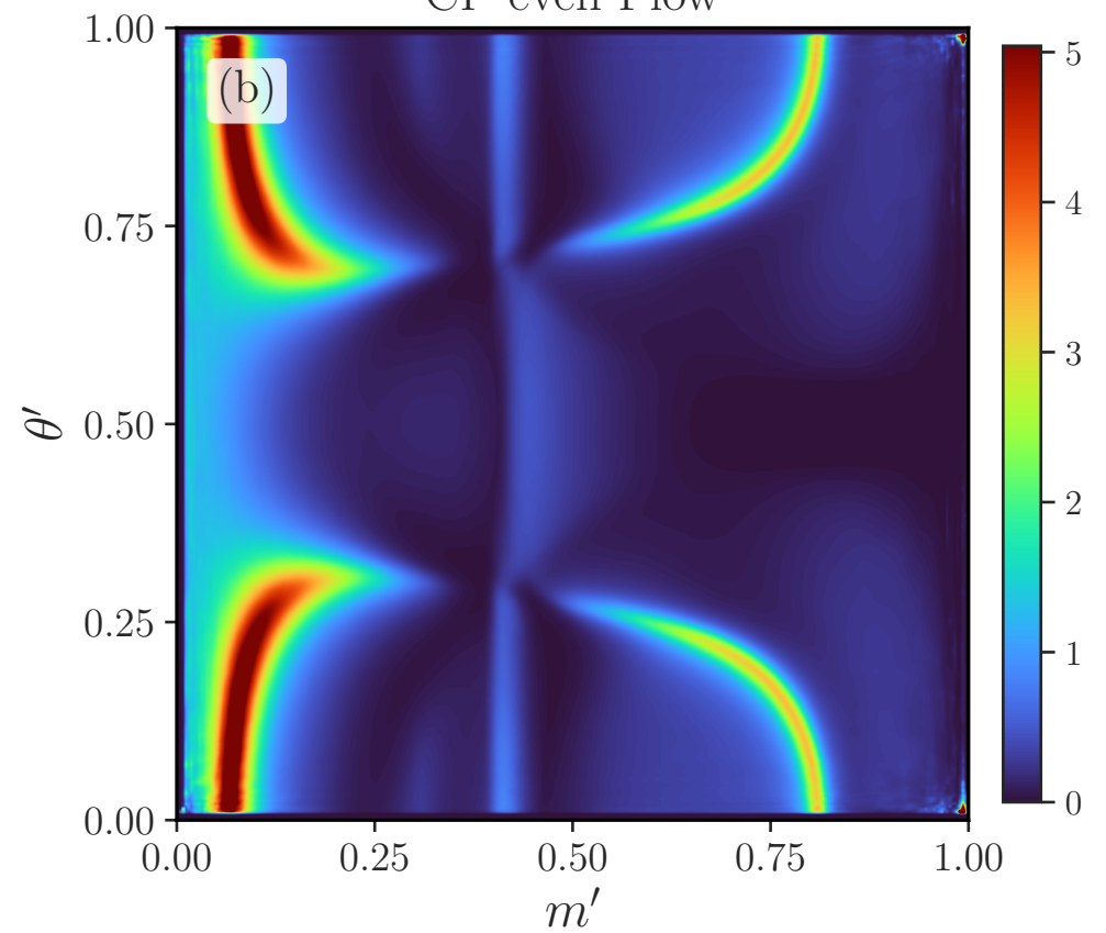
CP-even Flow
