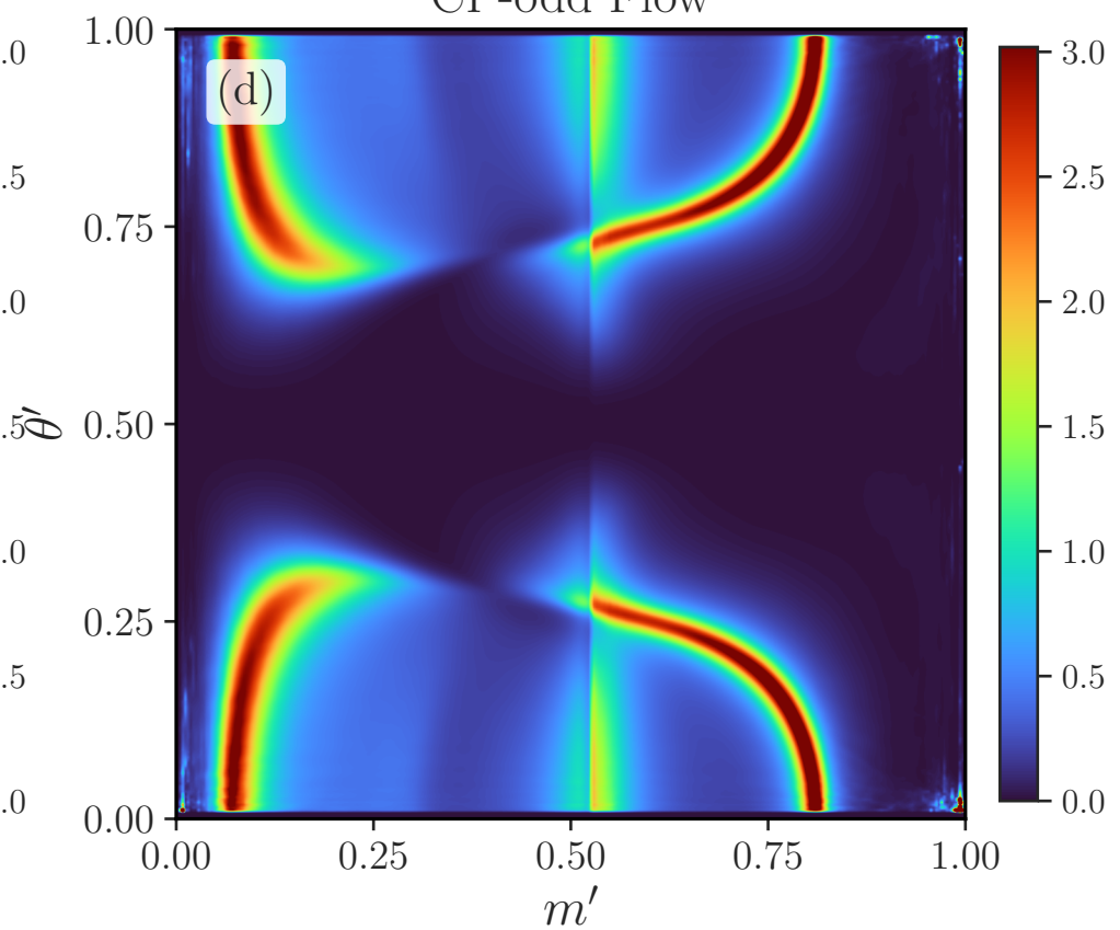
CP-odd Flow
