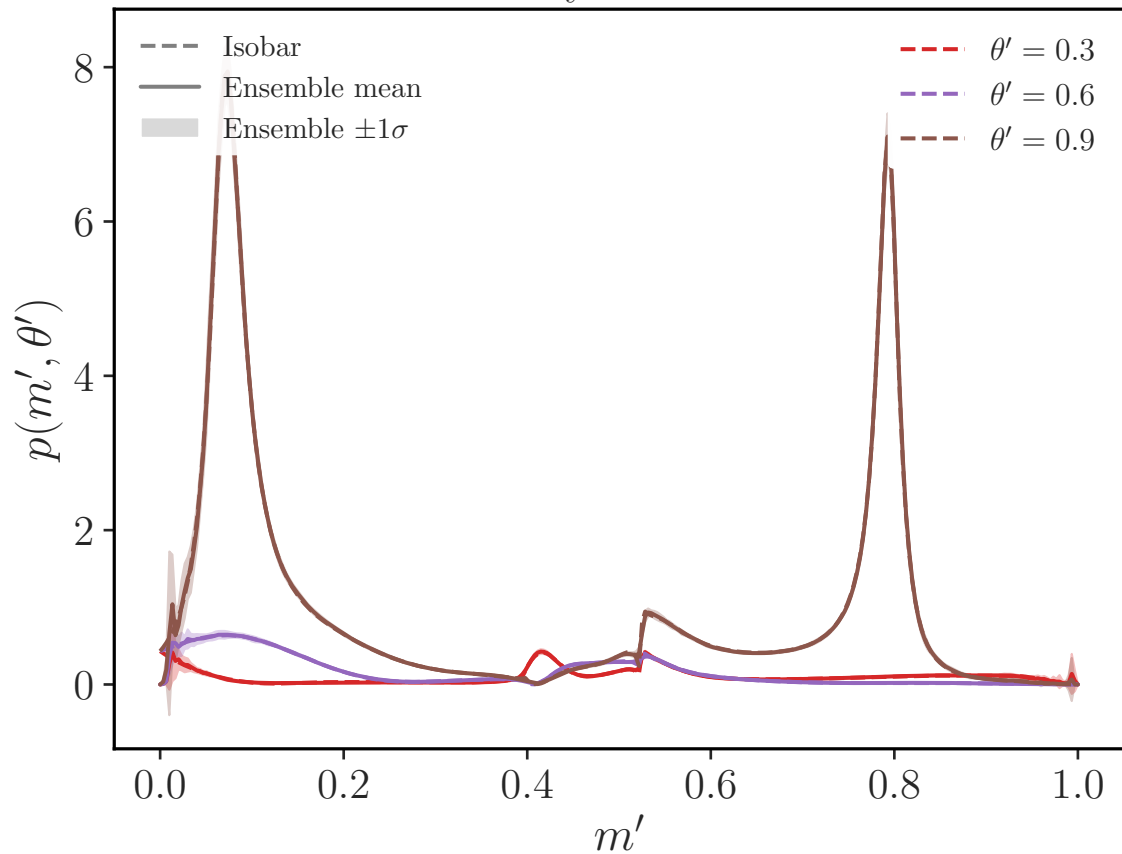
Density at fixed \theta'
