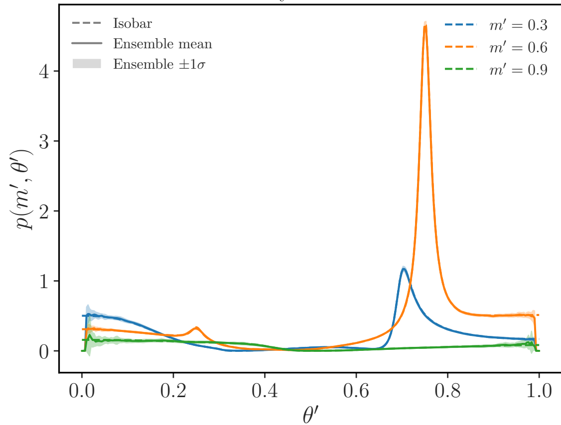
Density at fixed m'
