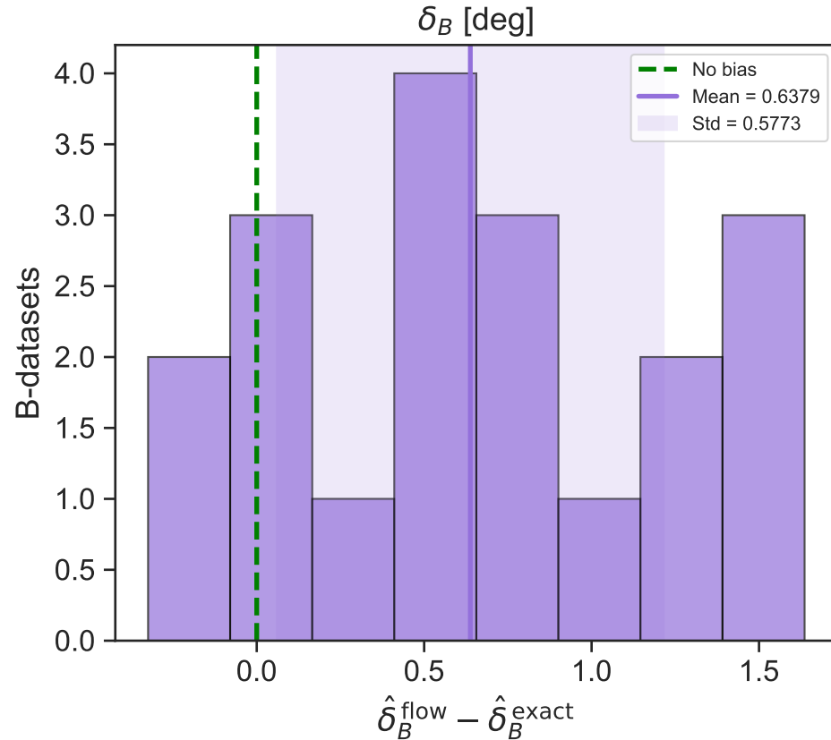
Flow model bias (flow – exact isobar) across 19 B-datasets
