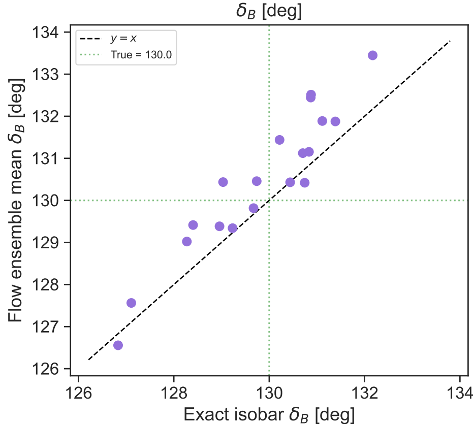
Flow ensemble mean vs Exact isobar (per B-dataset)
