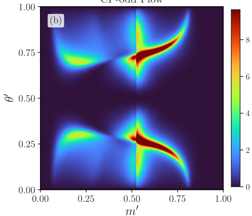
CP-odd Flow
