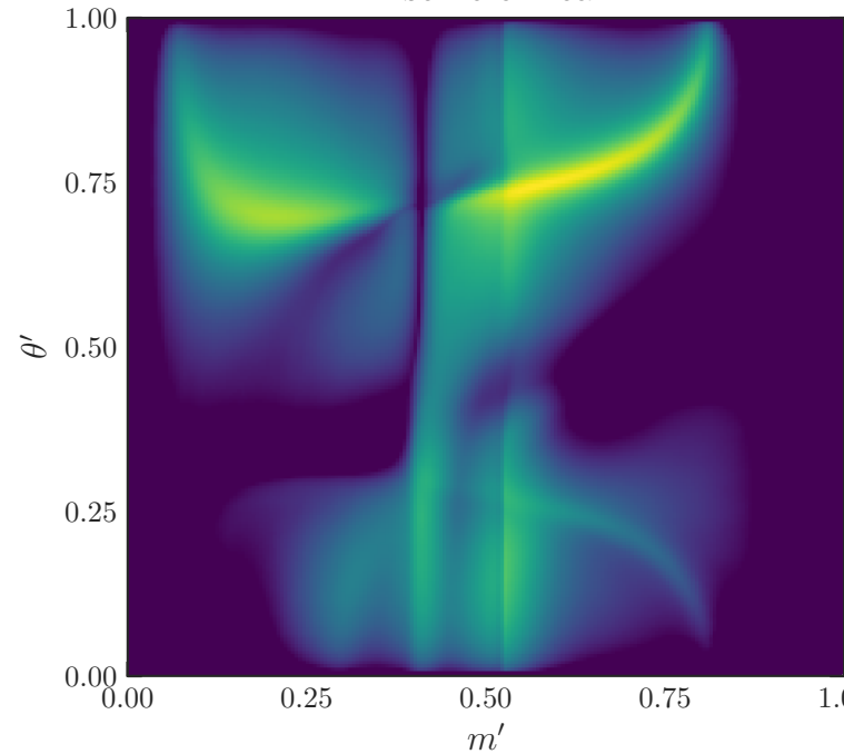
Ensemble mean
