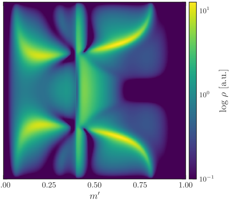
Exact isobar model
