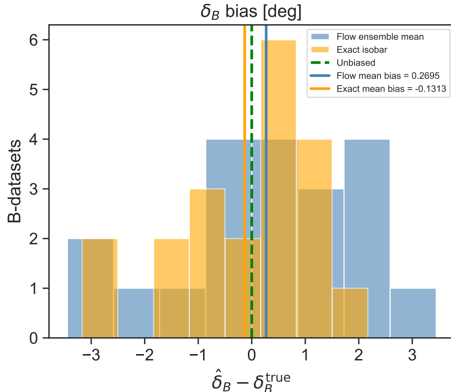
Bias across 20 B-datasets (Benchmark A, r_B = 0.1 )
