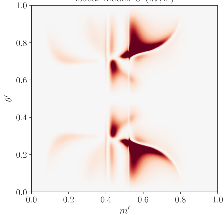
Isobar model: S^2(m', \theta')
