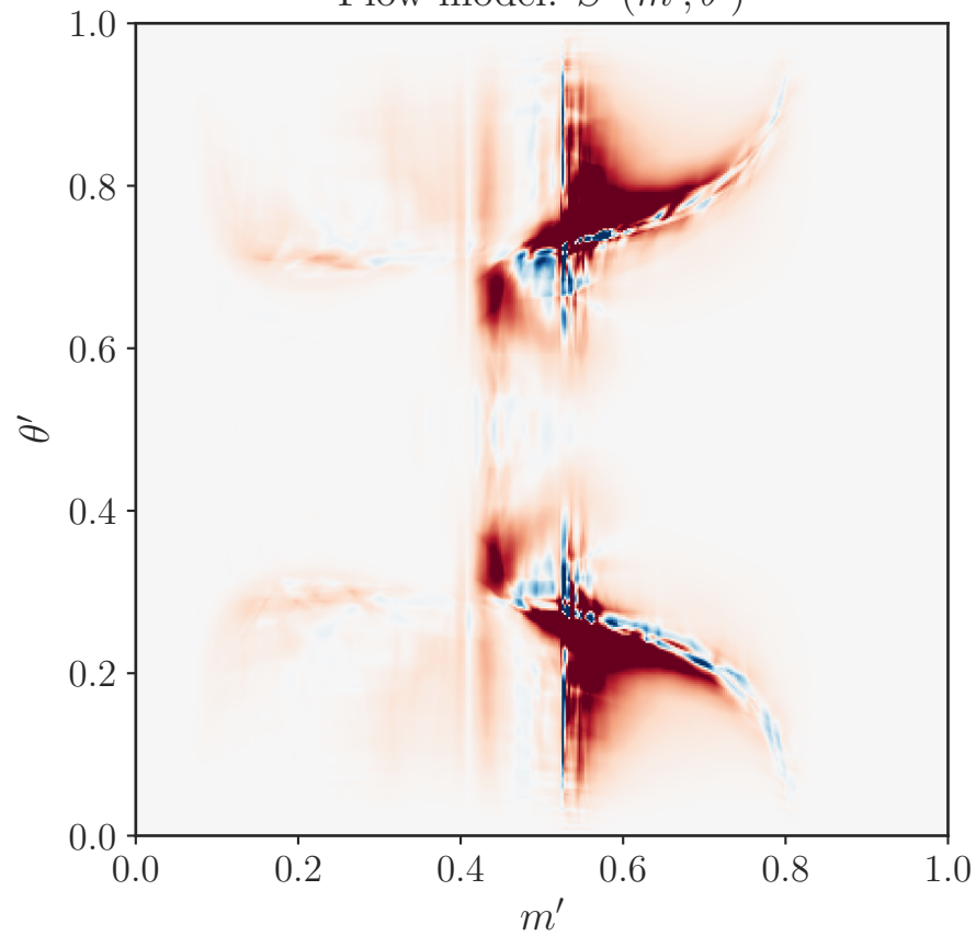
Flow model: S^2(m', \theta')
