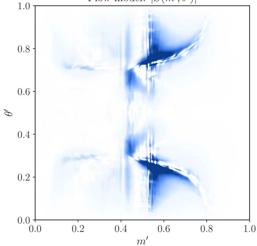
Flow model: |S(m', \theta')|
