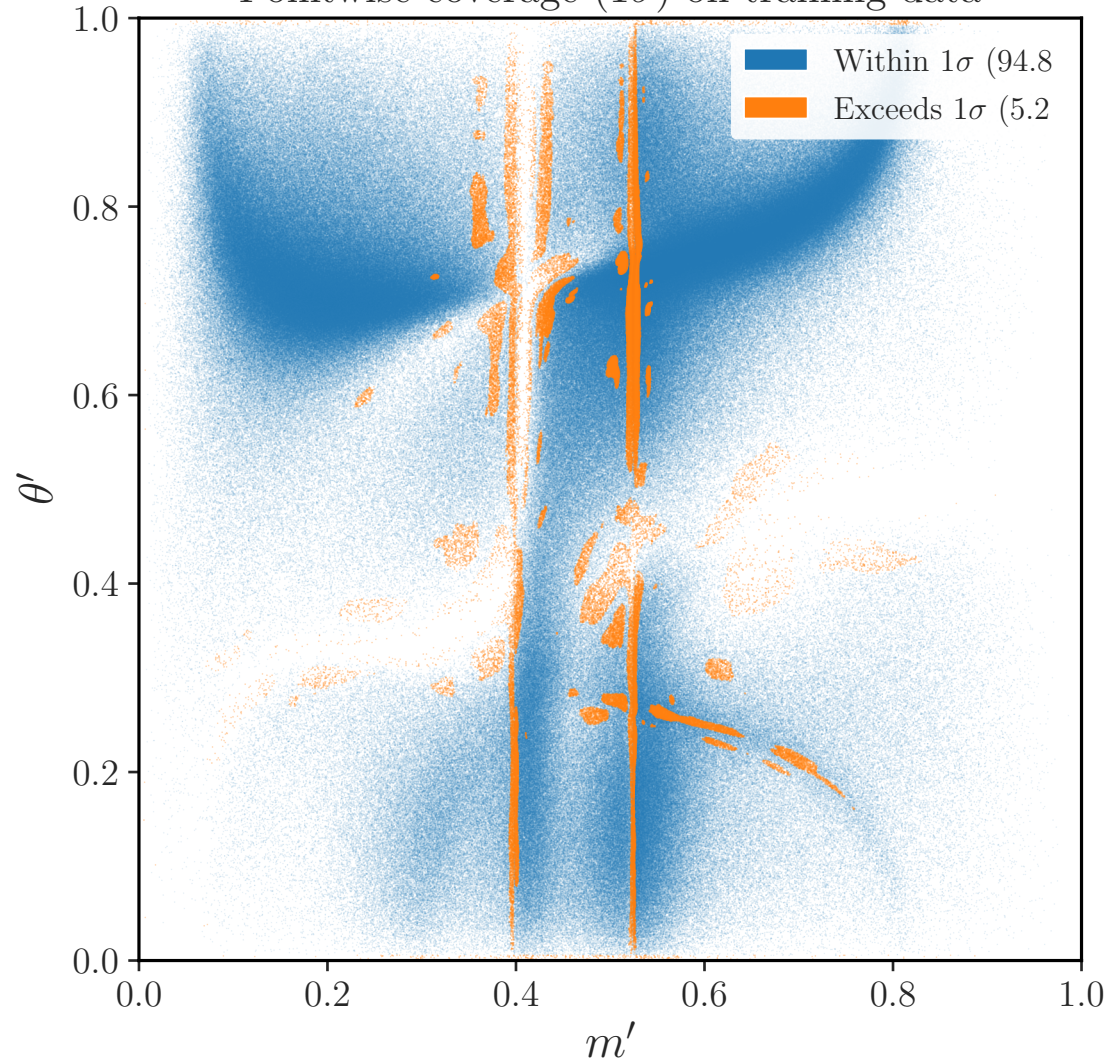
Pointwise coverage ( 1\sigma ) on training data
