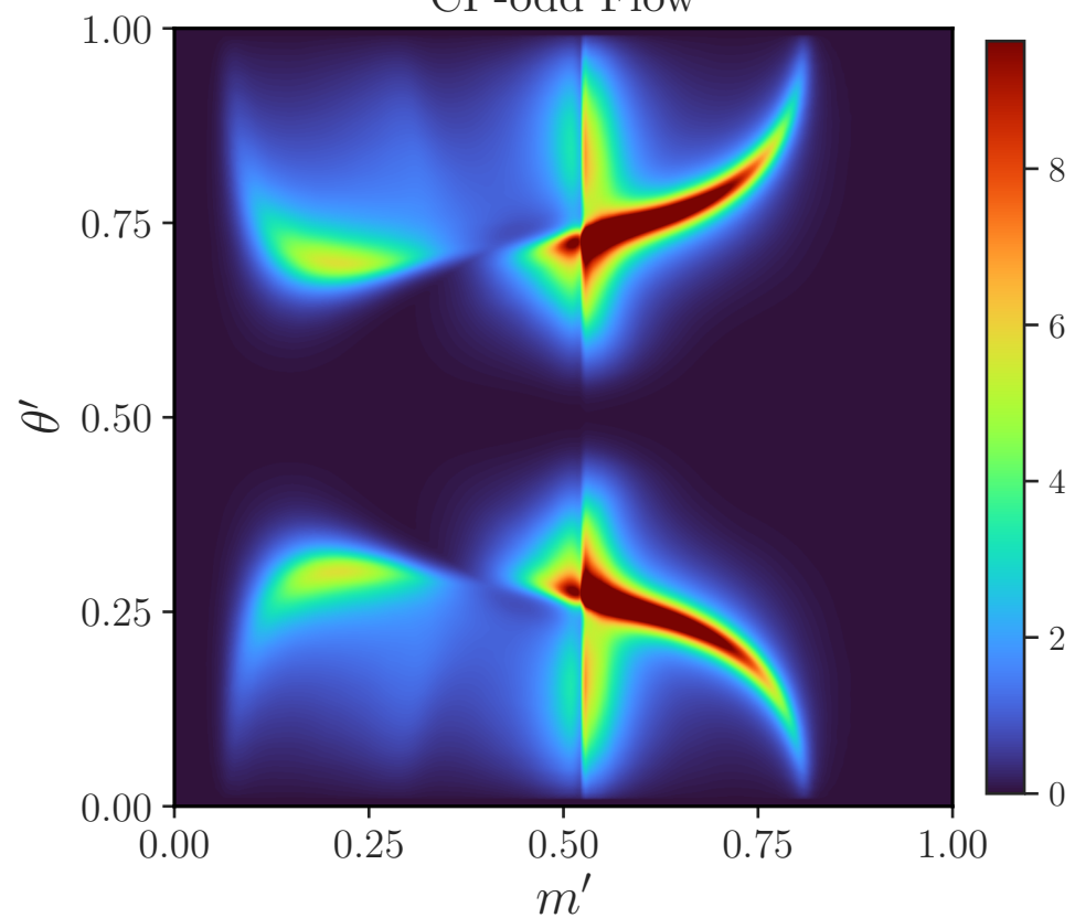
CP-odd Flow
