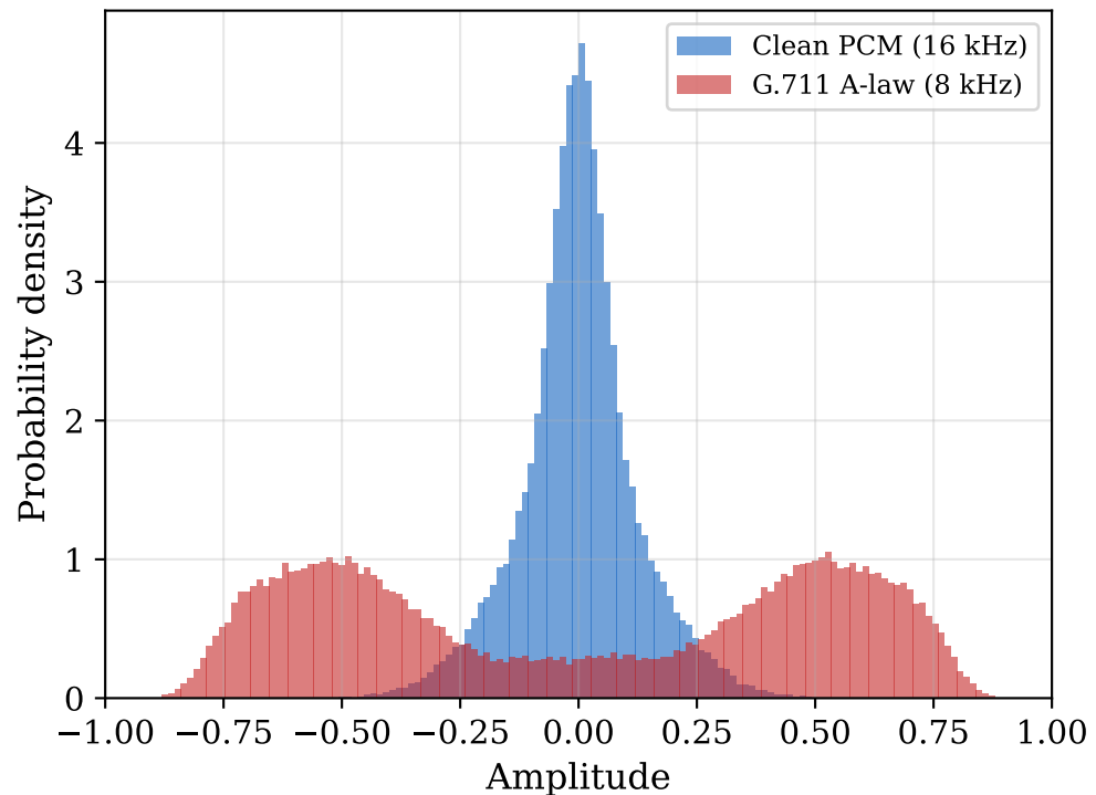
Amplitude Distribution Shift Clean PCM vs. G.711 A-law
