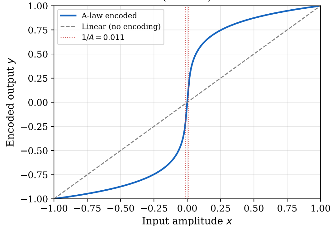
G.711 A-law Transfer Function ( A = 87.6 )
