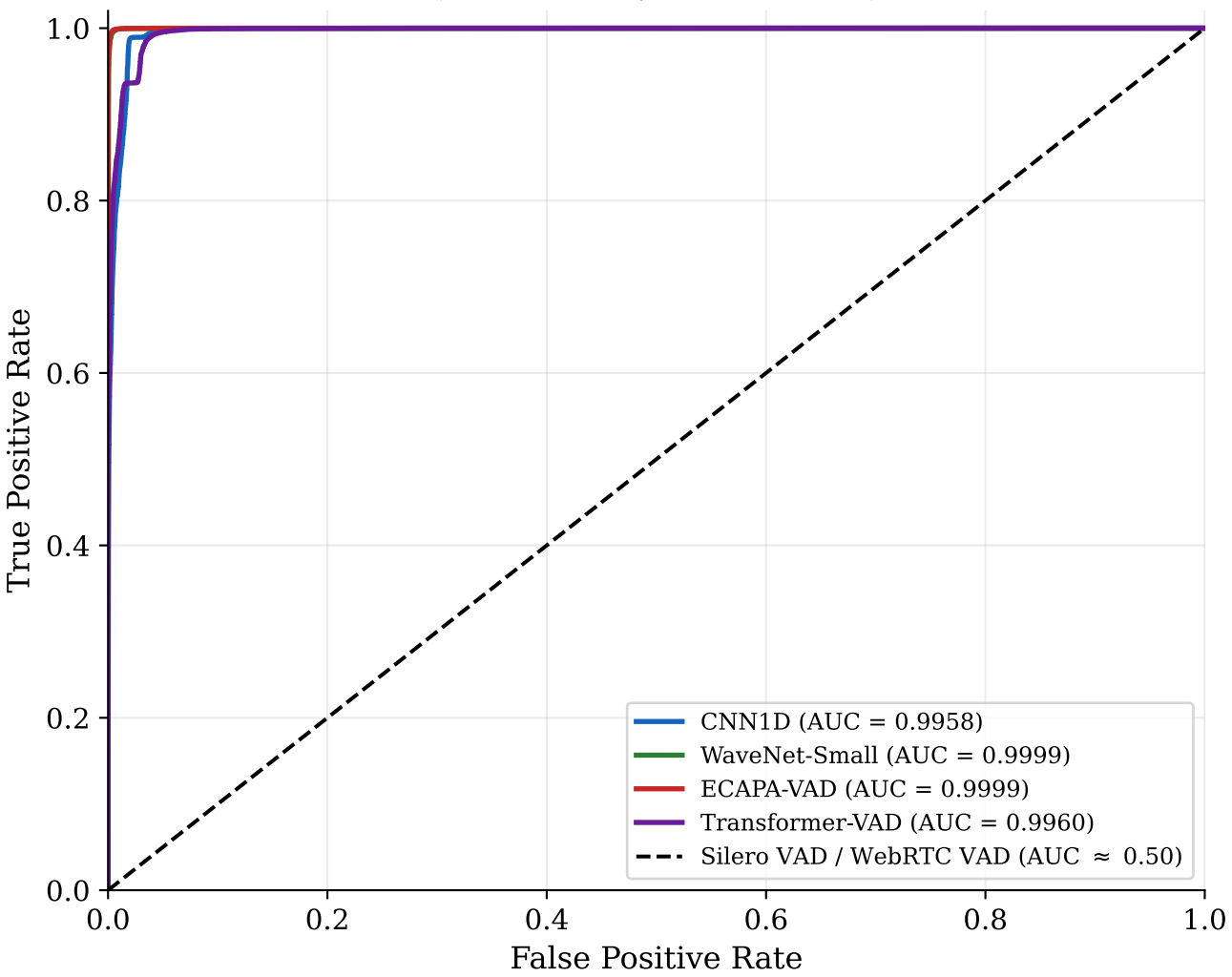
ROC Curves — G.711 A-law Trained Models (Test set: 60,000 windows)
