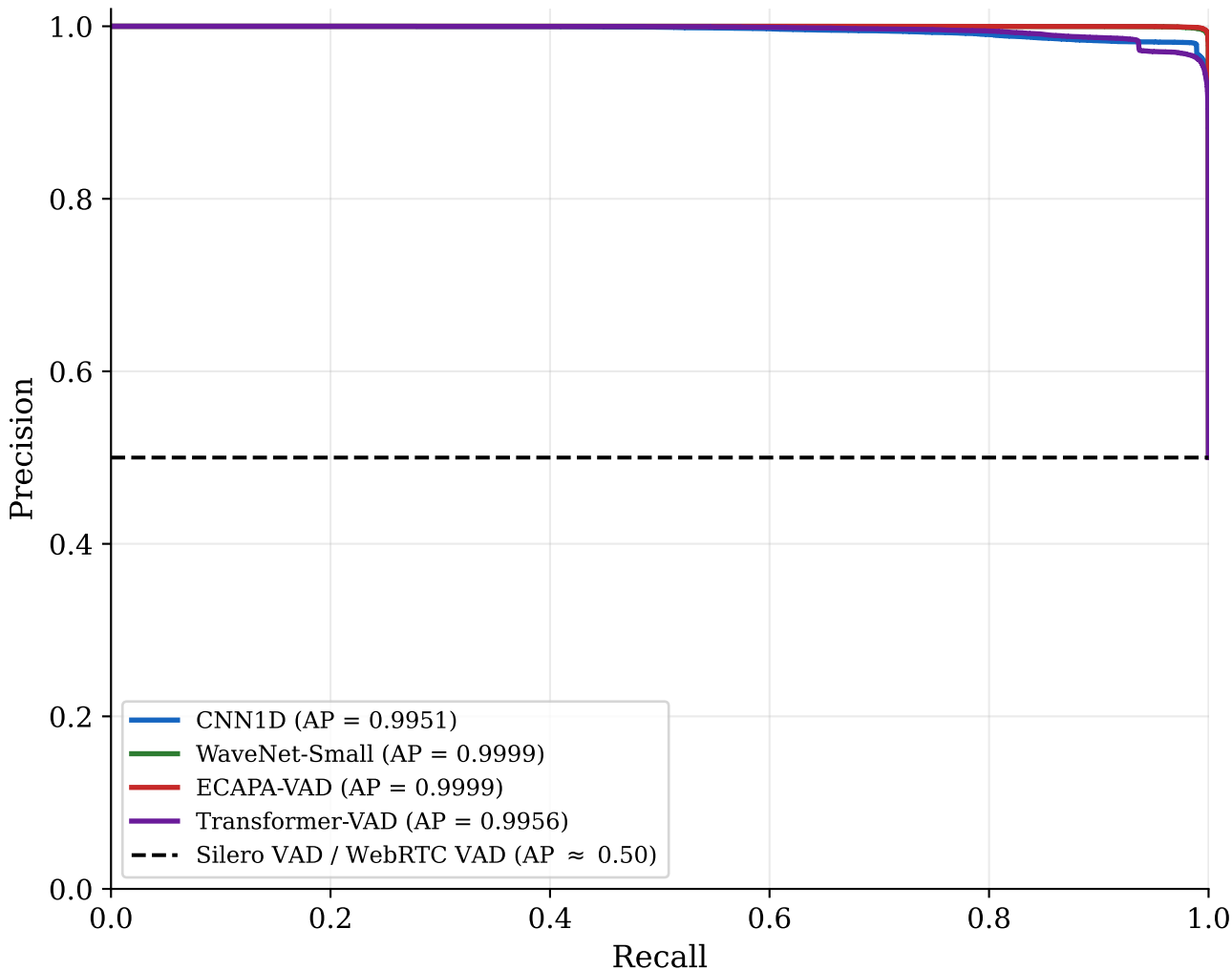
Precision-Recall Curves — G.711 A-law Trained Models (Test set: 60,000 windows)
