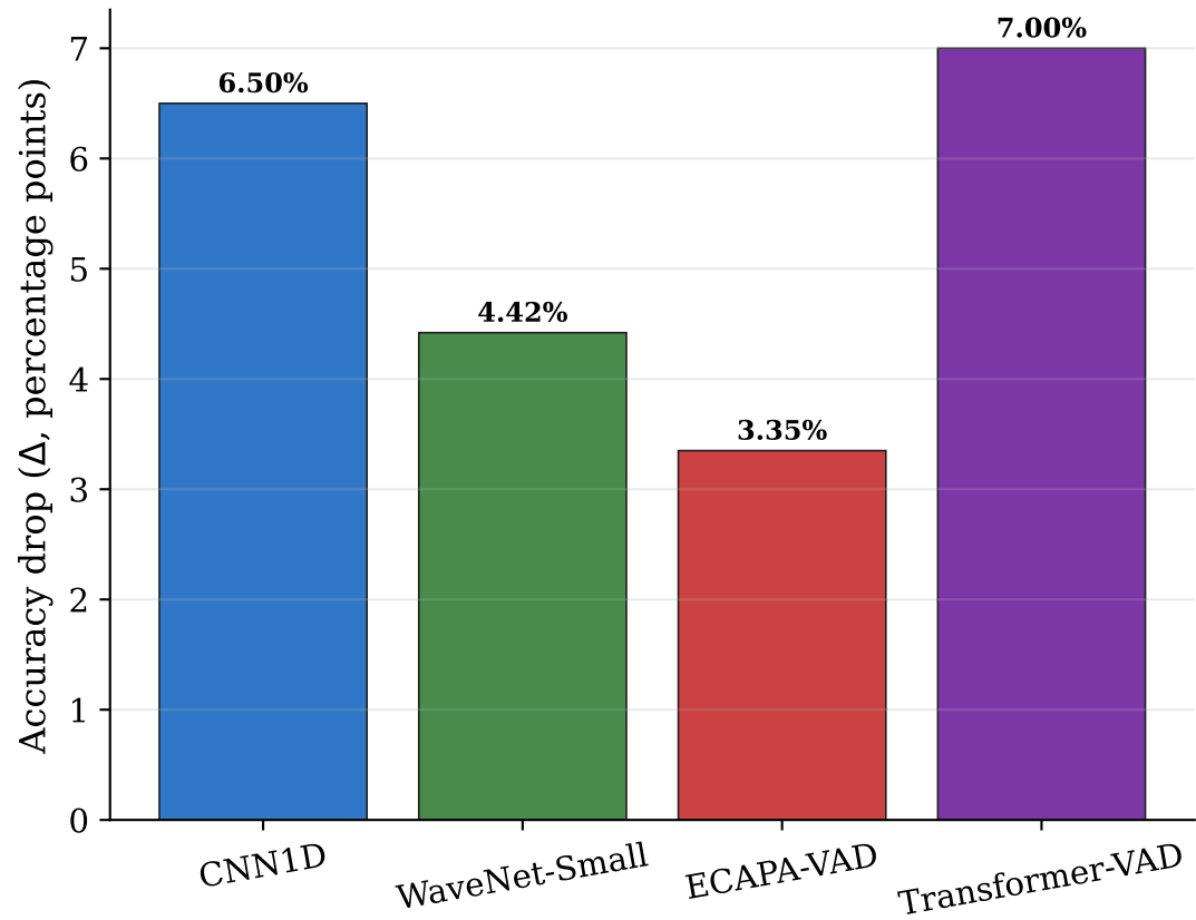
Codec-Induced Domain Gap ( \Delta = Own Acc – A-law Acc)
