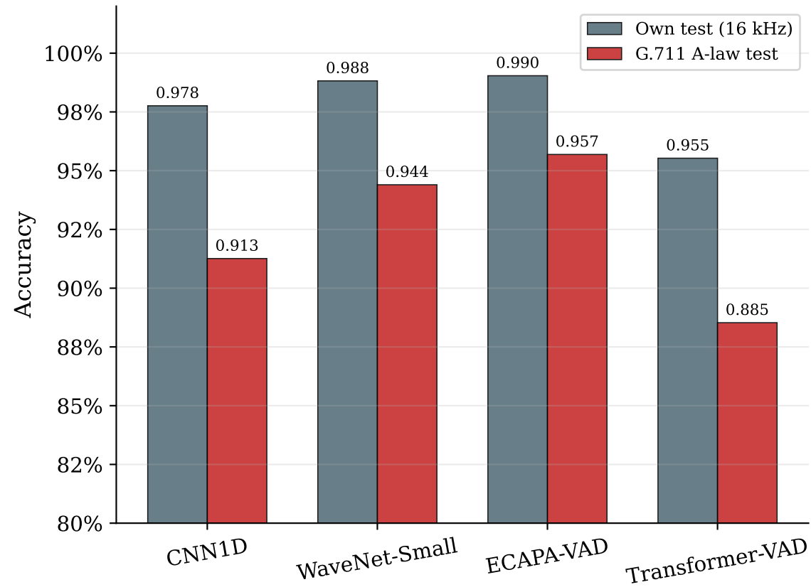
Own Test vs. G.711 A-law Test Accuracy (Raw 16 kHz trained models)
