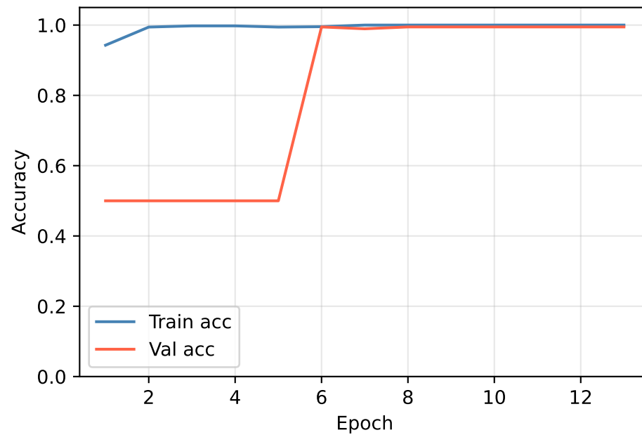
WaveNetSmall
