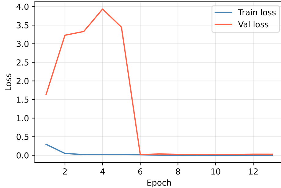
WaveNetSmall
