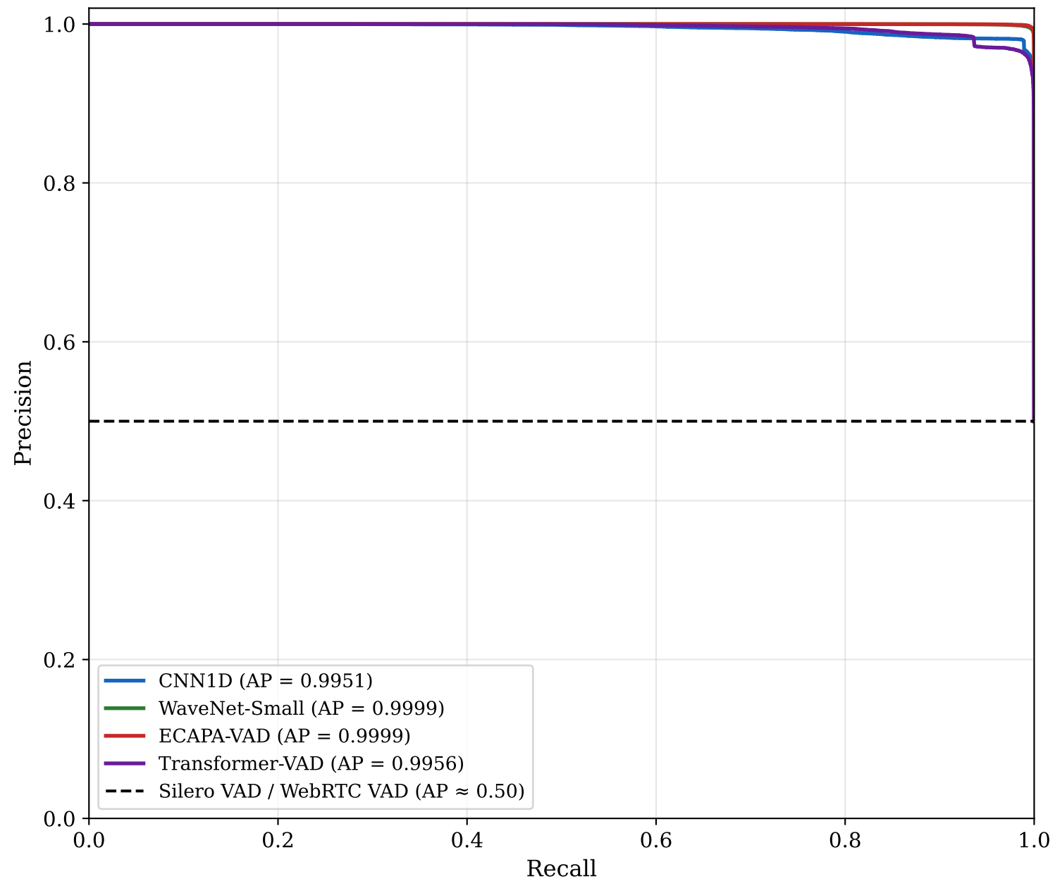
Precision-Recall Curves — G.711 A-law Trained Models
