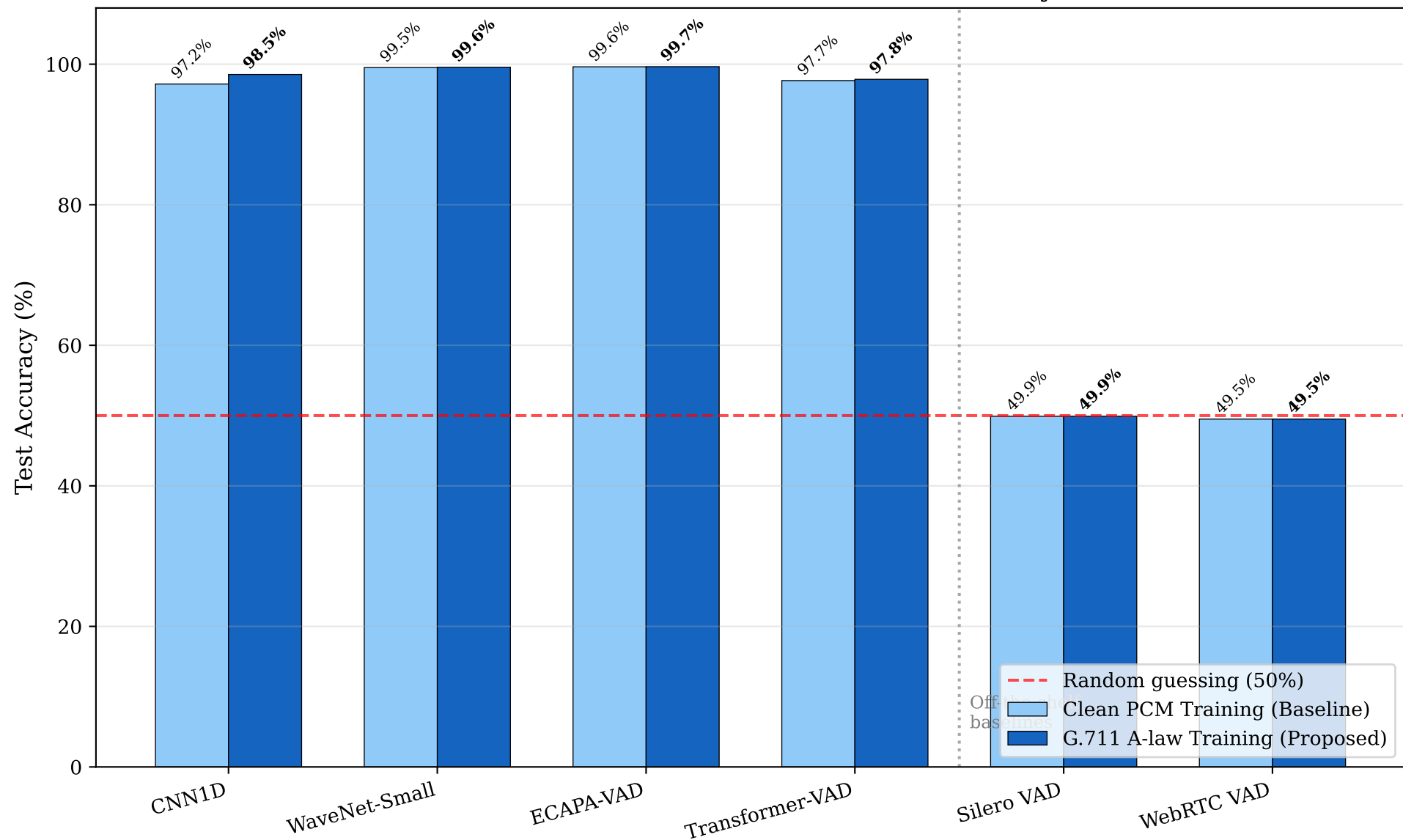
Test Accuracy Comparison: Proposed G.711-Compliant Training vs Clean PCM Baseline and Off-the-Shelf VAD Systems
