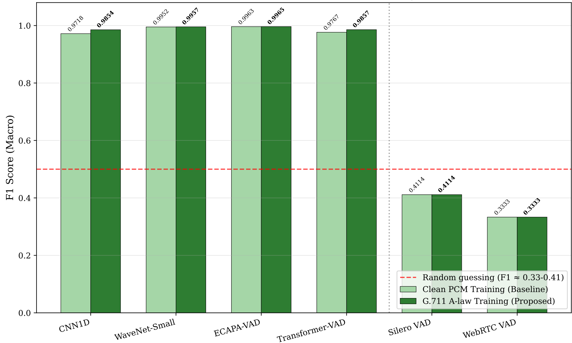
F1 Score Comparison Across Models and Training Conditions
