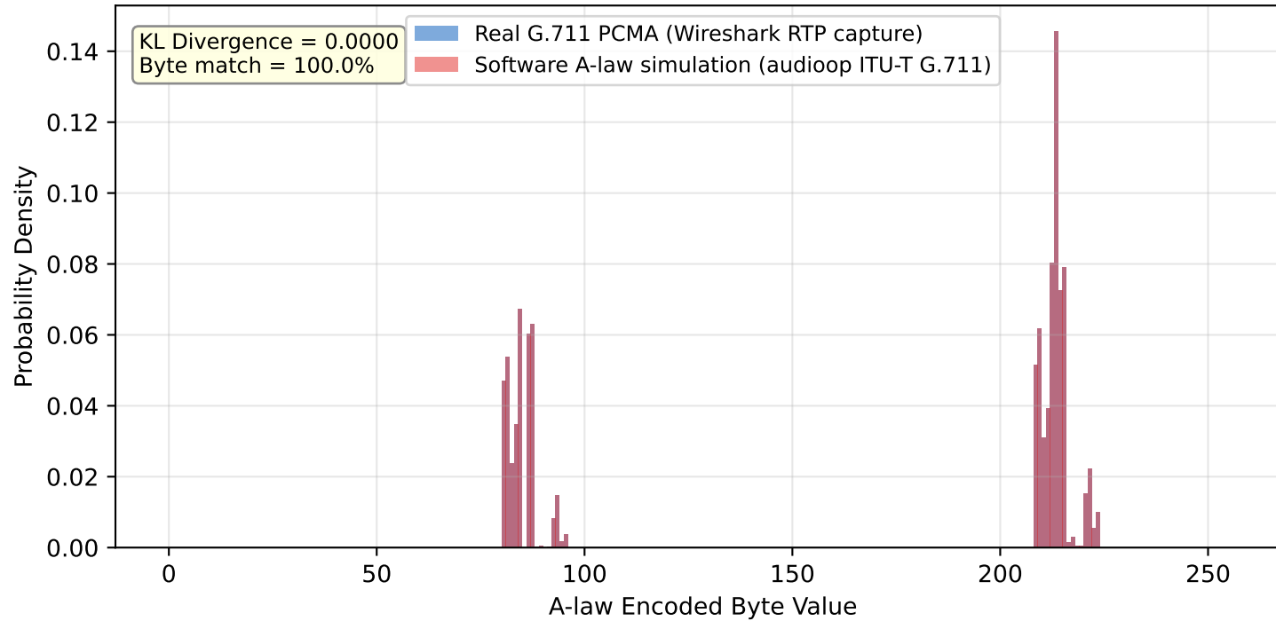
G.711 A-law Codec Output Byte Distribution
