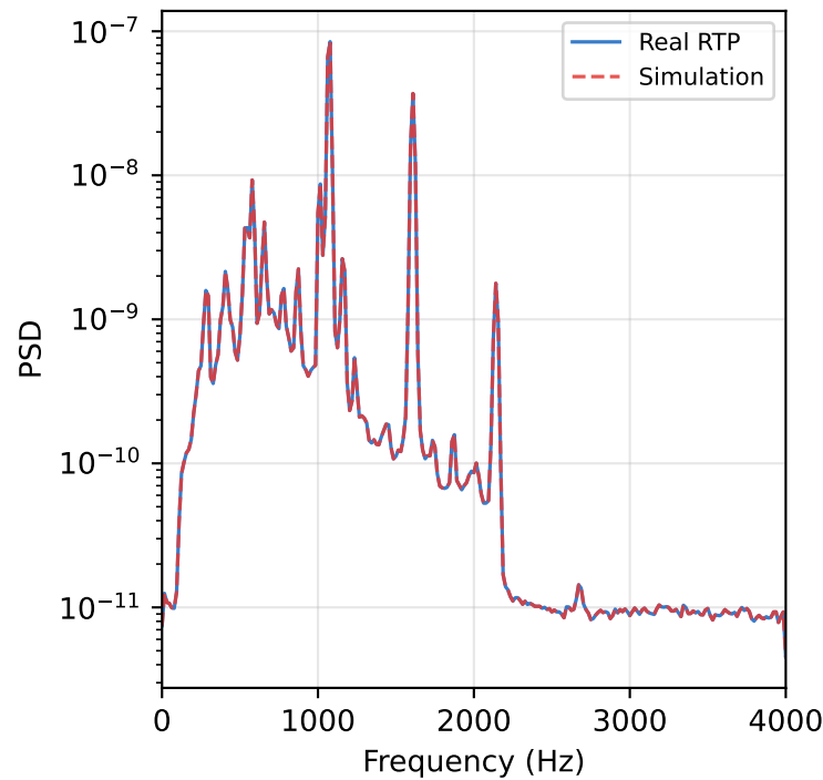
Power Spectral Density (0-4000 Hz bandwidth)
