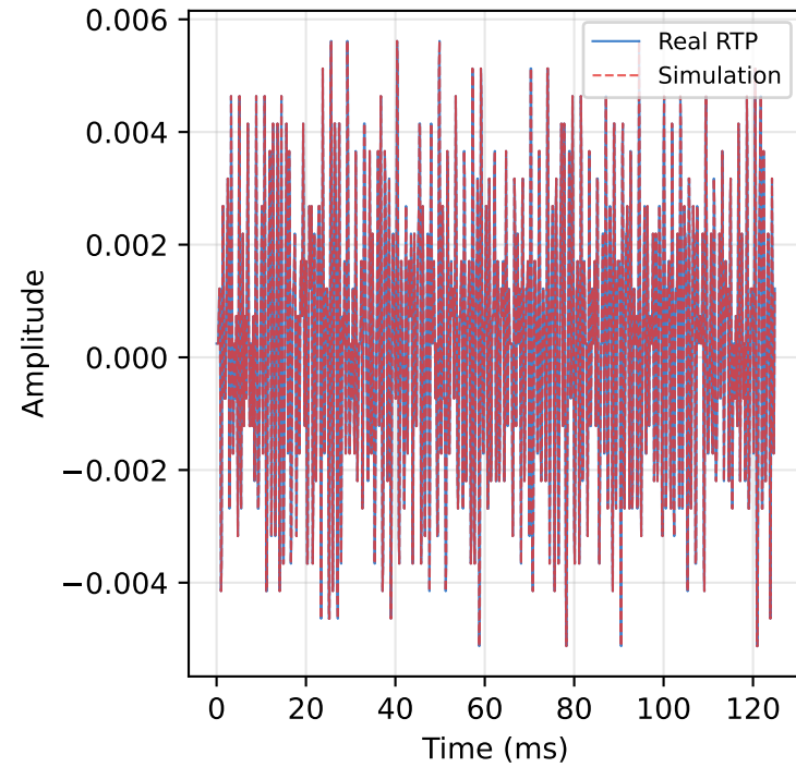
Decoded PCM Waveform (125ms window)
