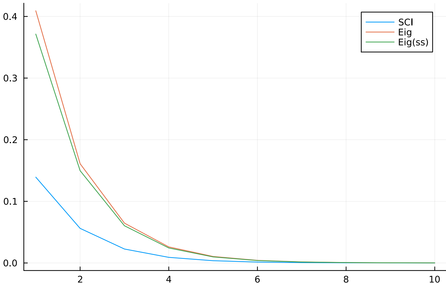
Expectation value of ZZI using SCI(R = 3) and Eigendecomposition of L for N=3
