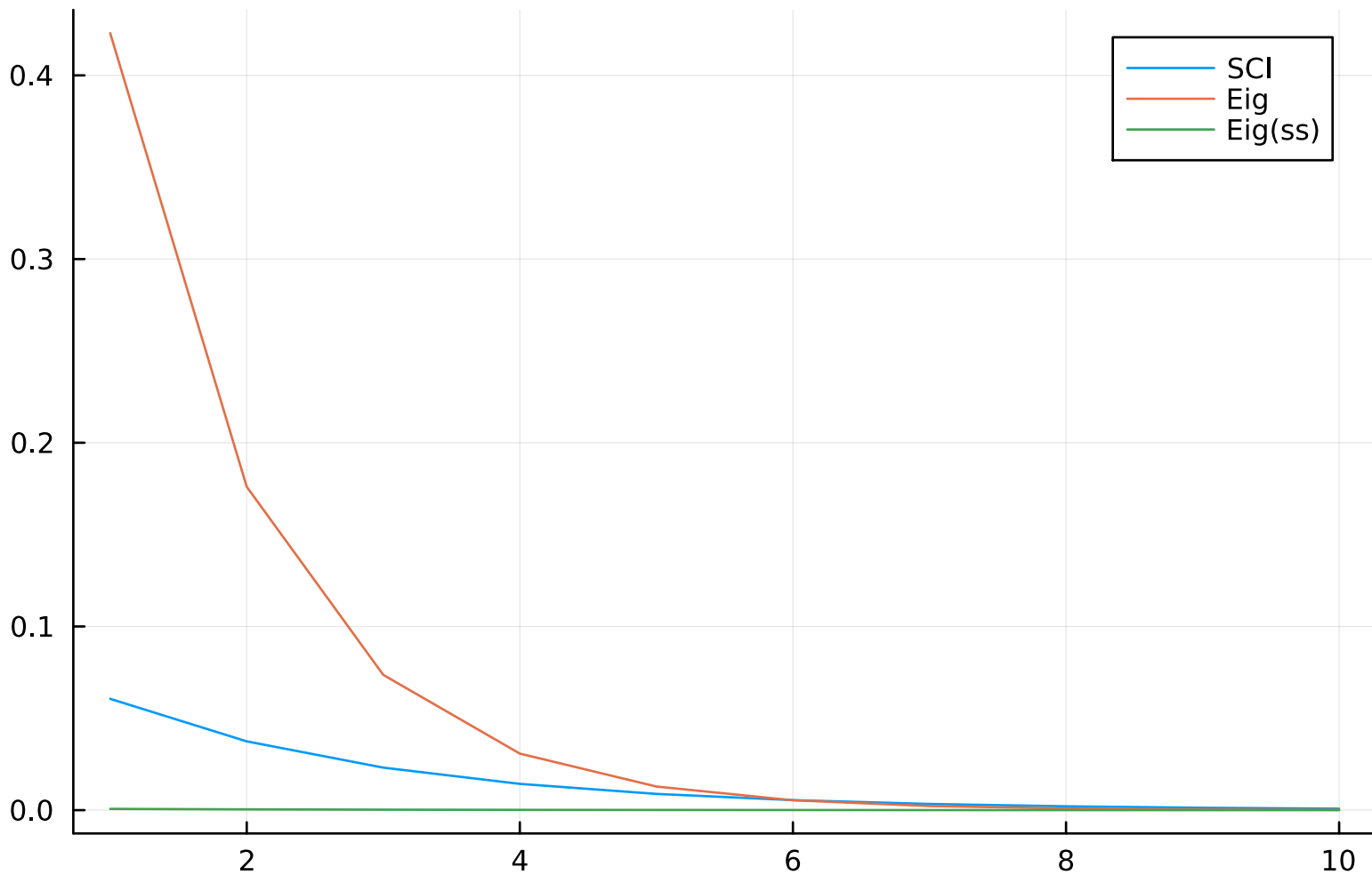
Expectation value of ZZIIII using SCI(R = 2) and Eigendecomposition of L for N=6
