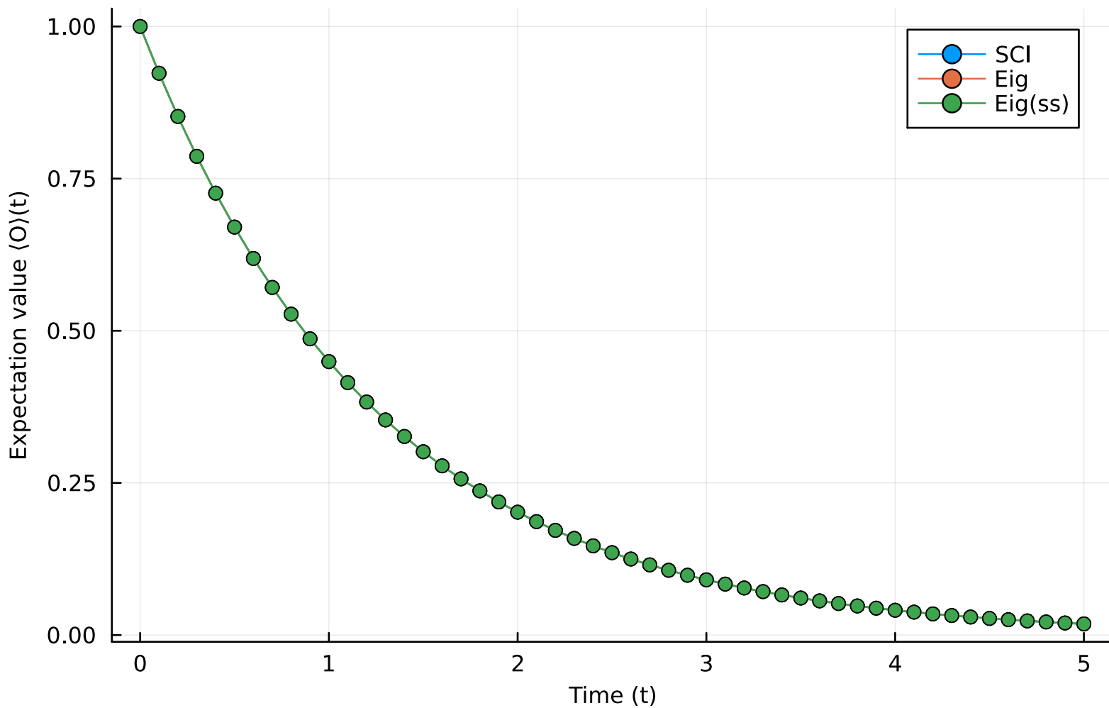
Expectation value of ZZ using SCI(R = 5) and Eigendecomposition of L for N=2
