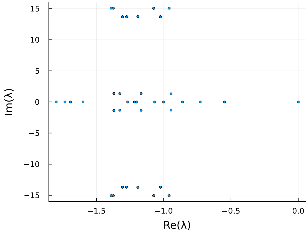
Full Diagonalization
