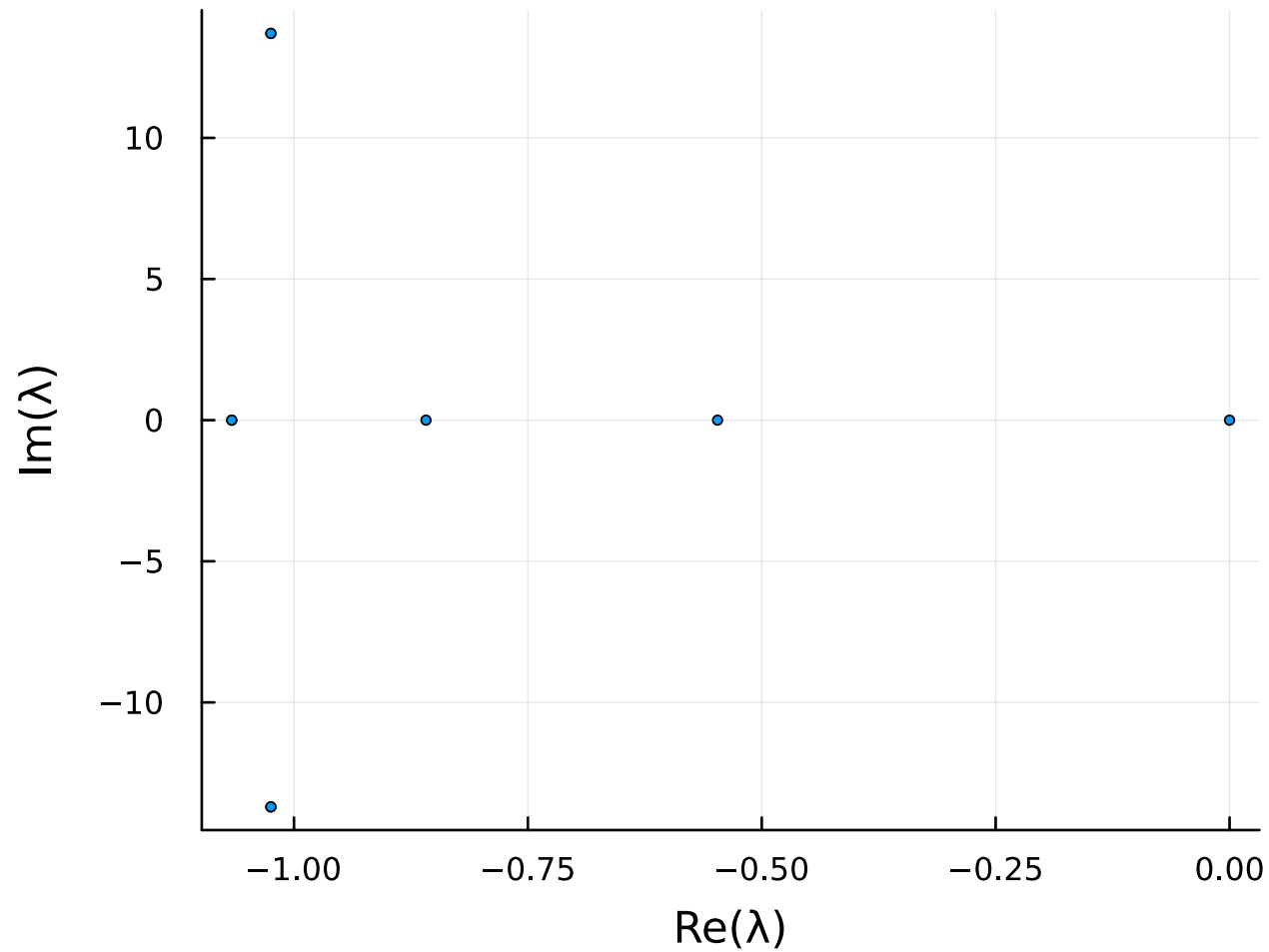
SCI Approximation
