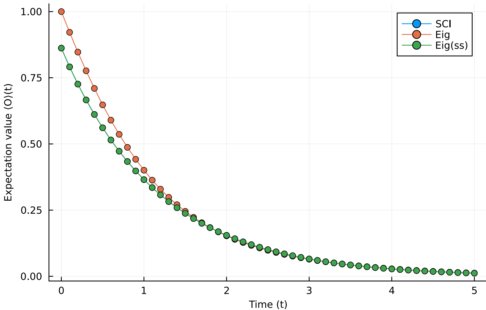
Expectation value of ZZI using SCI(R = 10) and Eigendecomposition of L for N=3
