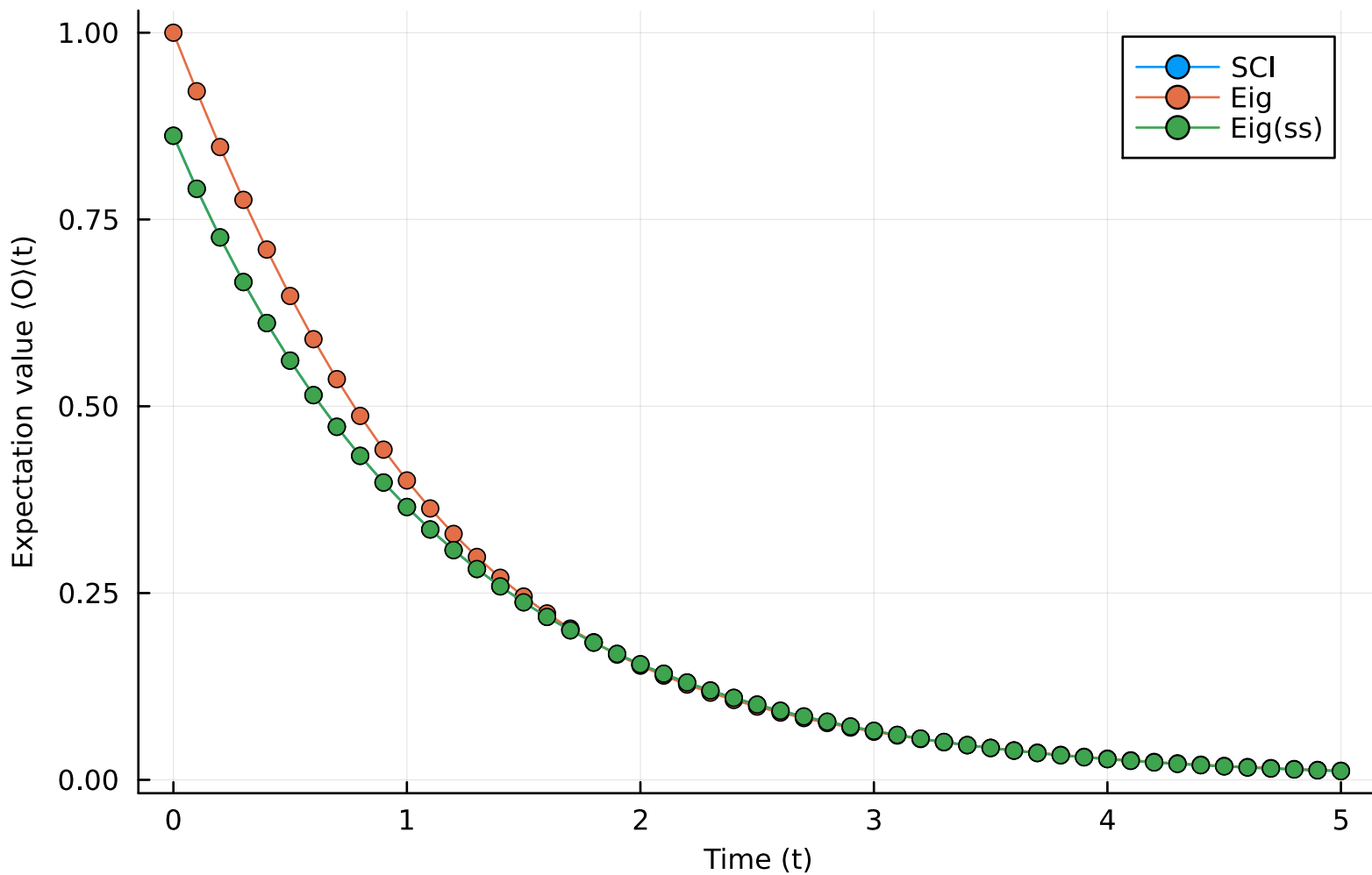
Expectation value of ZZI using SCI(R = 9) and Eigendecomposition of L for N=3
