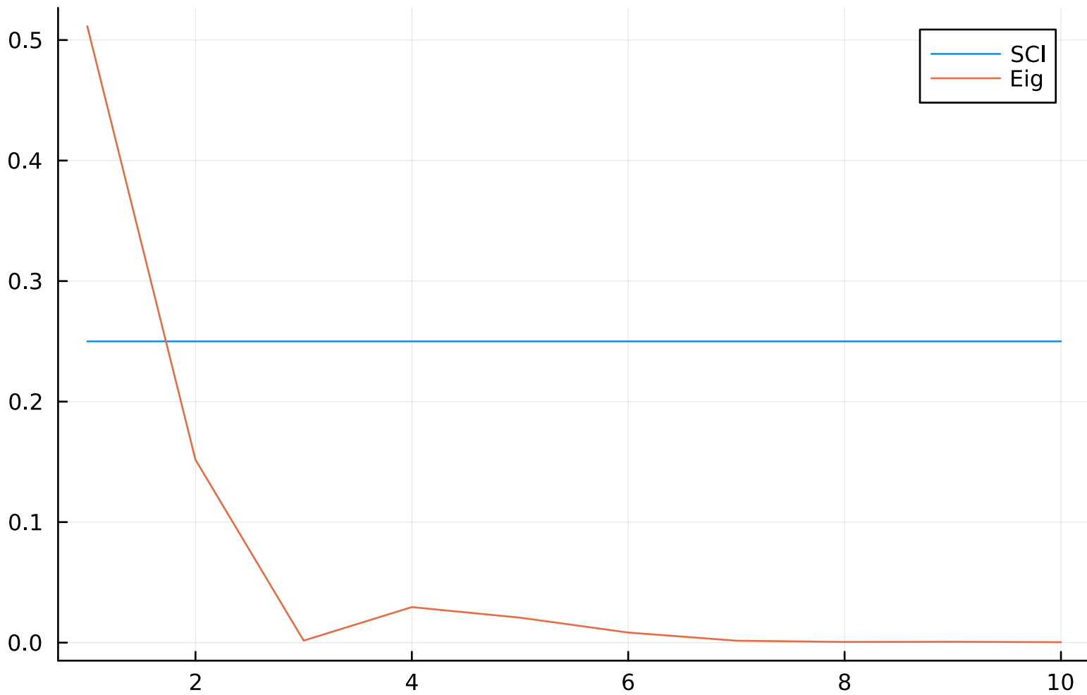
Expectation value of Z_1 using SCI( R = 2 ) and Eigendecomposition of L for N=2
