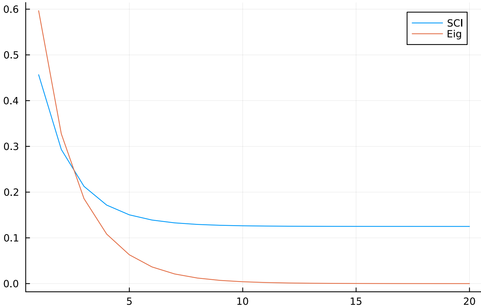
Expectation value of Z_1 using SCI( R = 10 ) and Eigendecomposition of L for N=3
