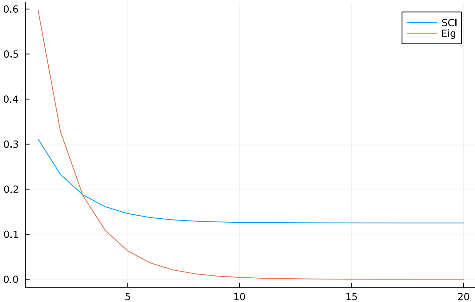
Expectation value of Z_1 using SCI( R = 2 ) and Eigendecomposition of L for N=3
