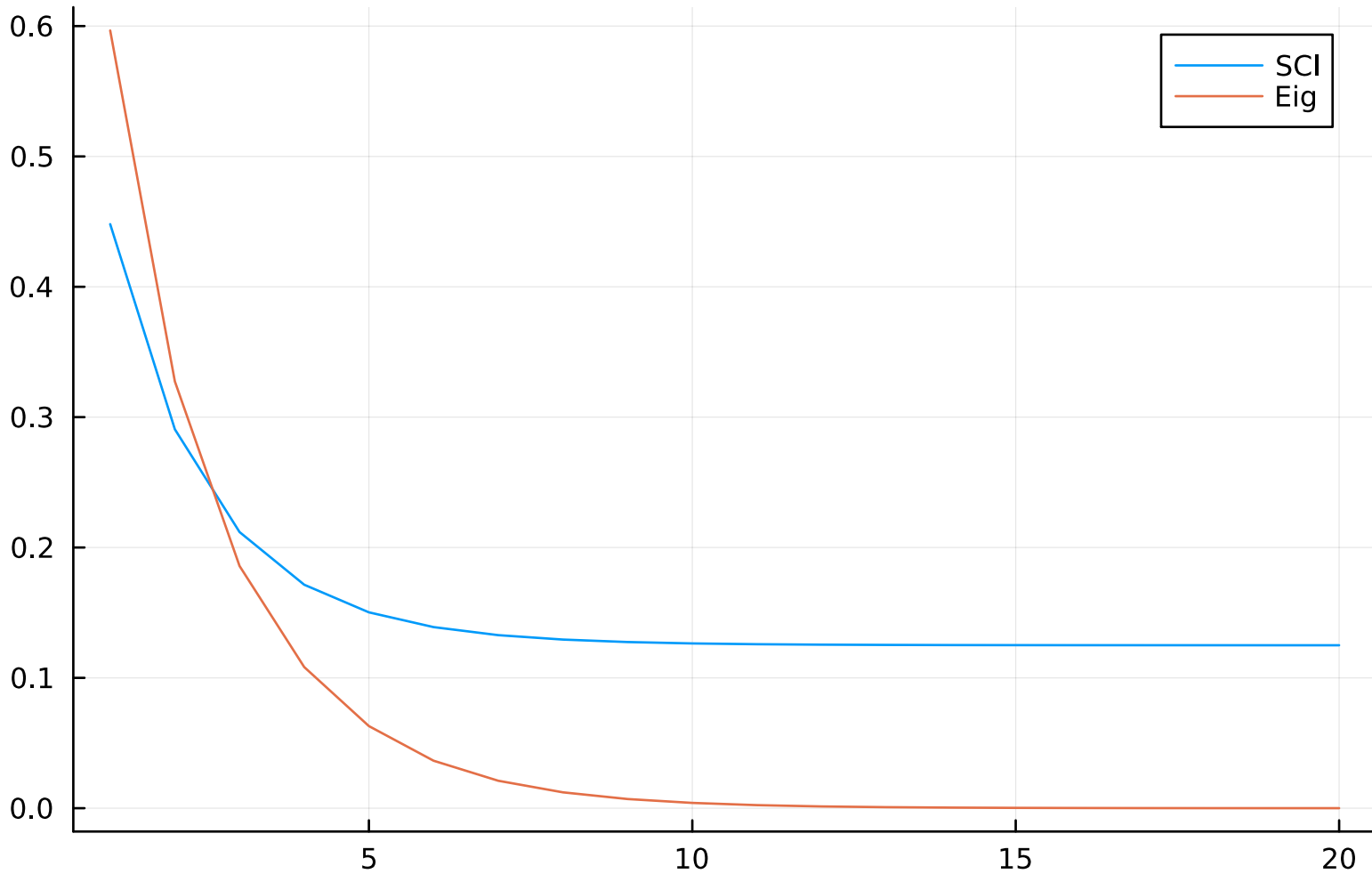
Expectation value of Z_1 using SCI( R = 5 ) and Eigendecomposition of L for N=3
