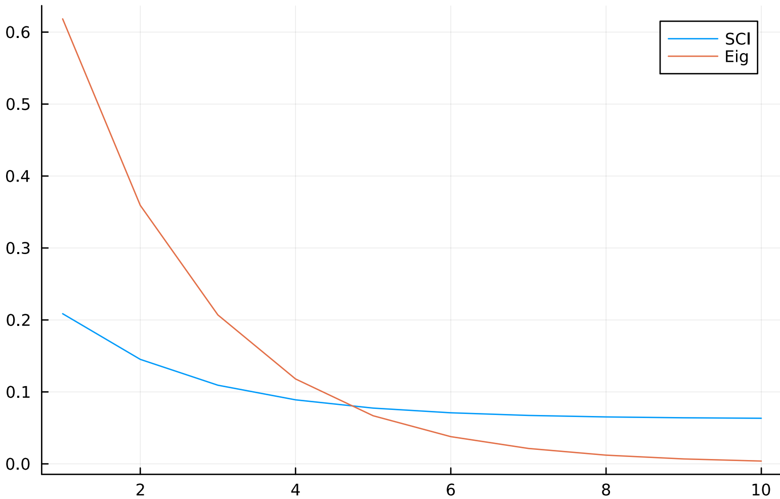
Expectation value of Z_1 using SCI( R = 2 ) and Eigendecomposition of L for N=4
