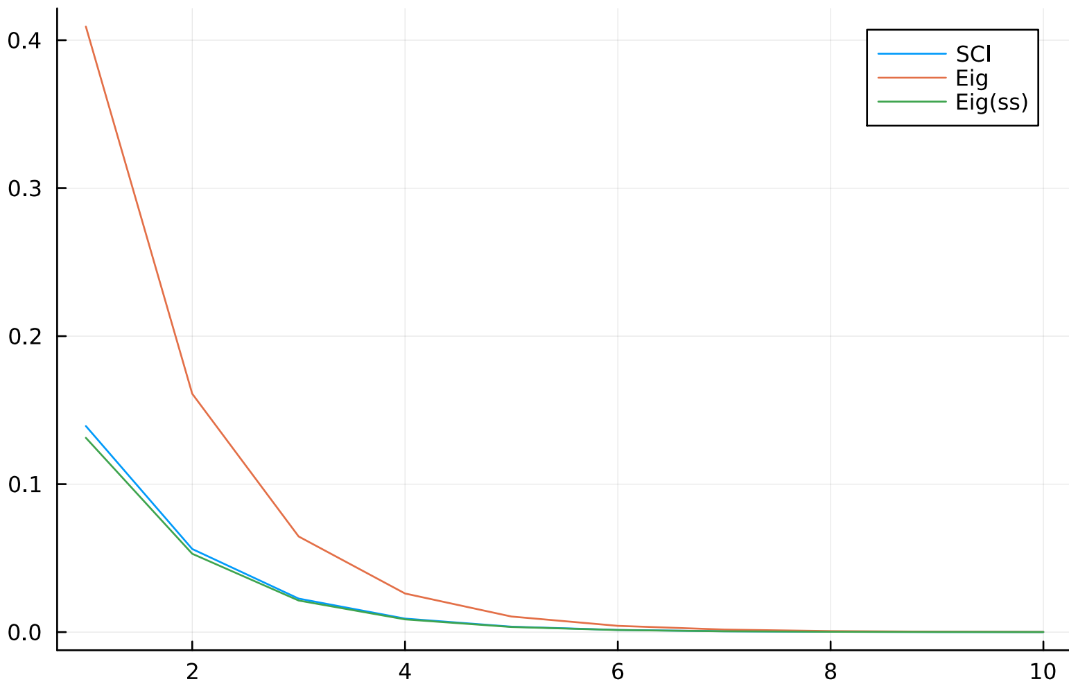
Expectation value of Z_1 using SCI( R = 3 ) and Eigendecomposition of L for N=3
