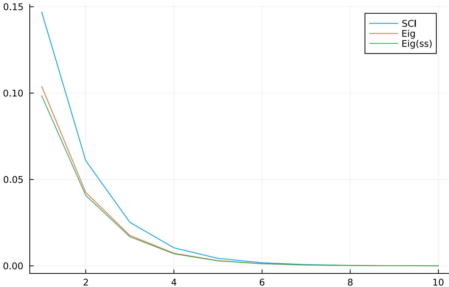
Expectation value of Z_1 using SCI( R = 3 ) and Eigendecomposition of L for N=4
