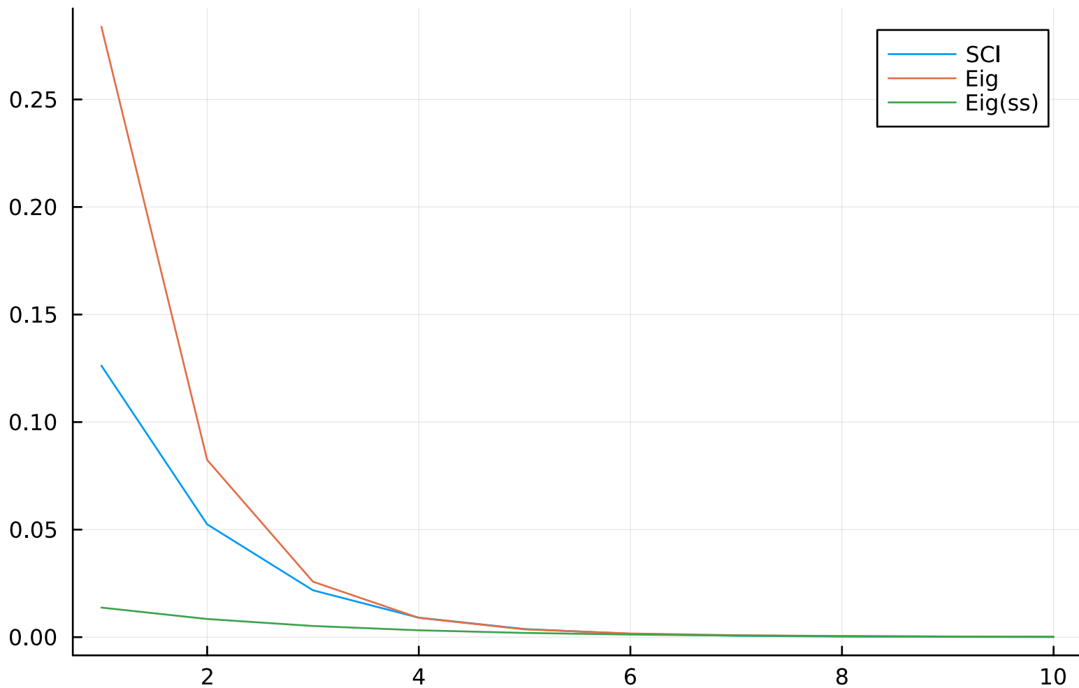
Expectation value of Z_1 using SCI( R = 3 ) and Eigendecomposition of L for N=5
