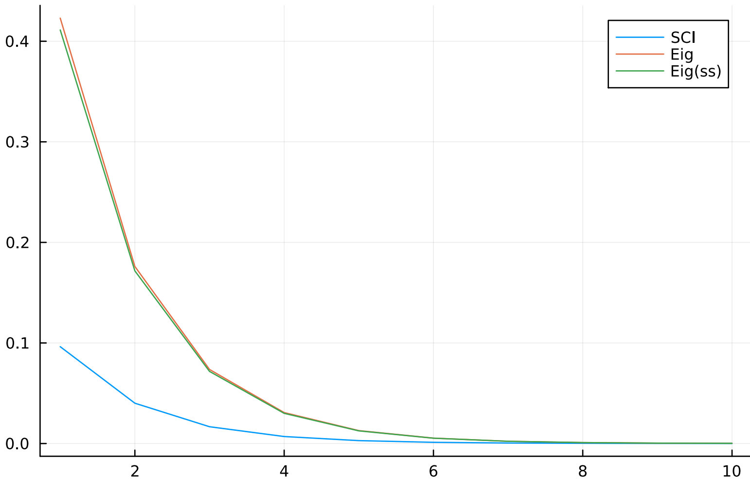
Expectation value of Z_1 using SCI( R = 3 ) and Eigendecomposition of L for N=6
