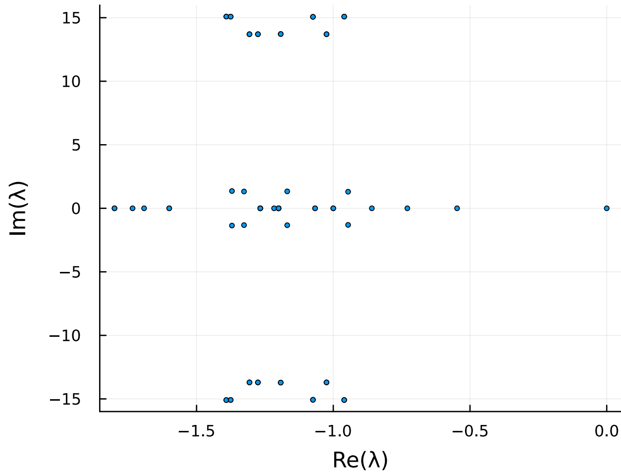
Full Diagonalization
