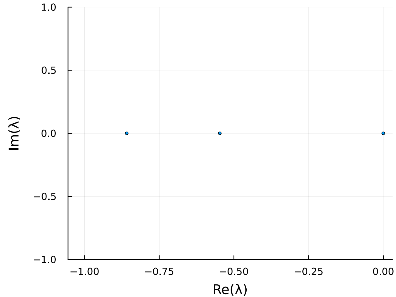
SCI Approximation
